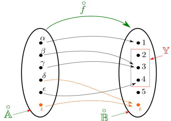
Fig. 3. Introduction of Not a Number \iota
