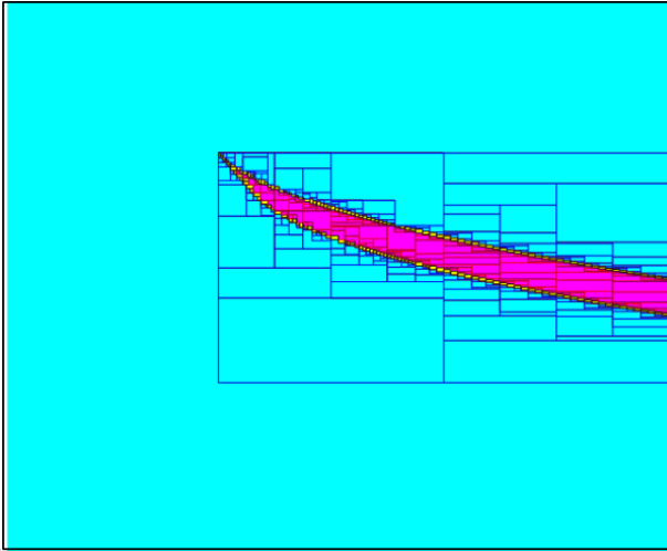
Fig. 6. Paving obtained using the contractor for \mathbb{S} and its complementary
