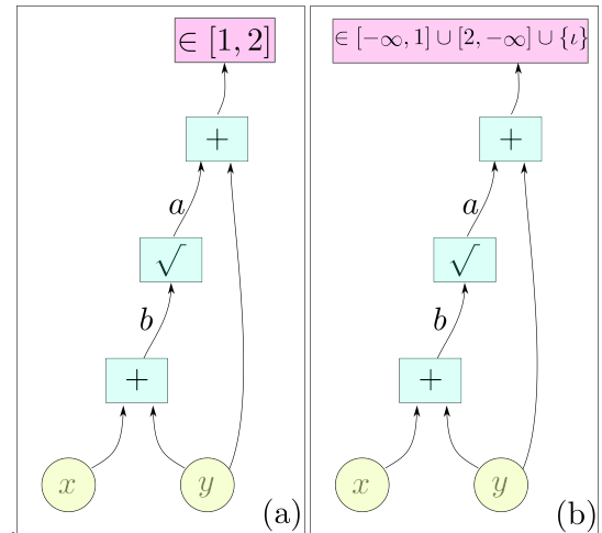
Fig. 5. AST for the constraint y + \sqrt{x+y} \in [1, 2] (left) and its complementary (right)
