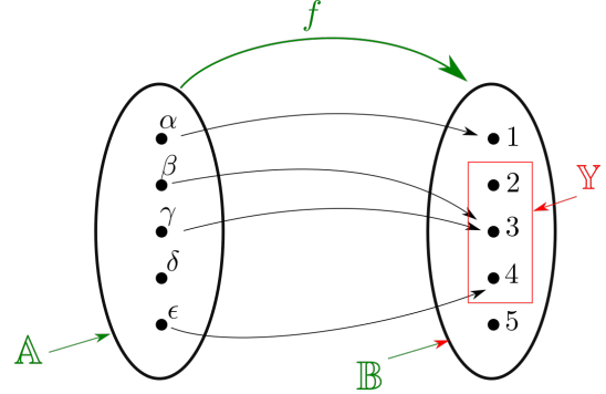
Fig. 2. A partial function f
