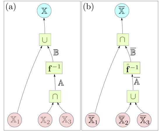
Fig. 1. (a) Contractor tree for \mathbb{X}_1 \cup \mathbf{f}^{-1}(\mathbb{X}_2 \cap \mathbb{X}_3) ; (b) its complementary
