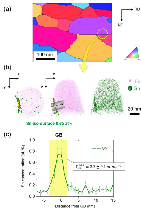
Figure 8: The ternary alloy prior to cold rolling a) EBSD ND-IPF mapping of the microstructure (black lines representing GBs with 15 – 65° misorientation), b) different views of the APT volume with Sn segregation (green spheres) at the prior GB, c) the concentration profile for Sn perpendicular to the interface.
