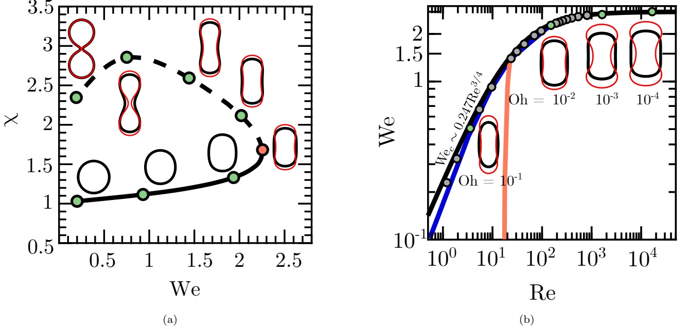
FIG. 2: Bifurcation diagram. (a): variation of the bubble elongation with the Weber number for a fixed value of the Ohnesorge number, here Oh = 10^{-2} ; (b) variation of the critical Weber number with the Reynolds number.
