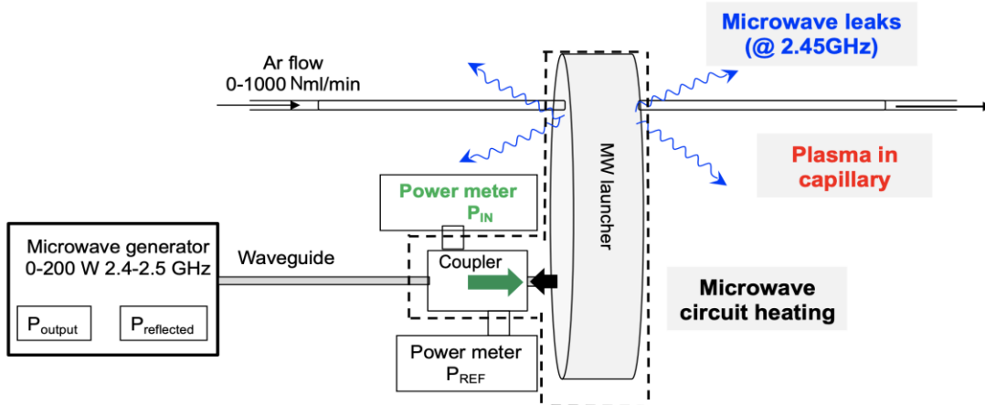
Figure 1. Schematics of the microwave capillary discharge set-up. The power difference ( P_{IN} - P_{REF} ) measured close to MW launcher is shared into the heat dissipated by the microwave circuit, the capillary plasma and microwave leaks.
