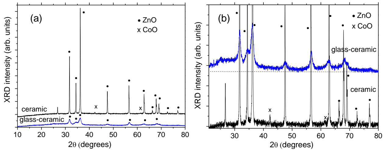
Fig. 231. XRD patterns of the ZnO glass-ceramics doped with 0.1% CoO prepared by the heat-treatment at 750 °C for 2 h and the ZnO:1 wt% Co (a); a close look on the XRD pattern of the ZnO glass-ceramics doped with 0.1% CoO prepared by the heat-treatment at 750 °C for 2 h (b).
