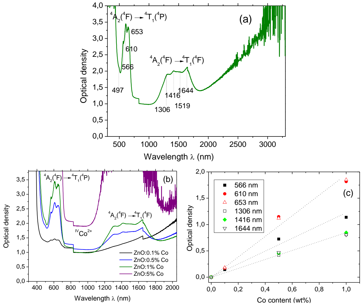
Fig. 2220. Absorption spectrum of ZnO:1 wt% Co ceramic in the spectral range of 300 – 3300 nm (a); absorption spectra of ZnO: Co ceramics doped with 0.1 – 5.0 wt.% Co in the spectral range of 300 – 2050 nm (b); the dependence of the the peak optical density at 566, 610, 653, 1306, 1416, and 1644 nm on the Co content (c). The thickness of the samples is \sim 0.5 mm.
