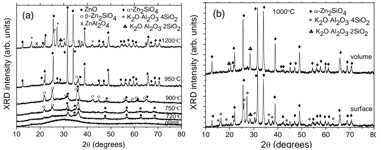
Fig. 6. XRD patterns of the glass Zn1 doped with 0.05% CoO. Heat-treatment temperatures are listed in the figure. Heat-treatment time is 2 h.
