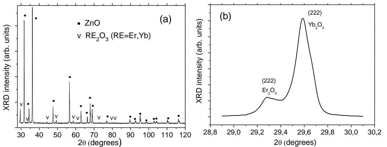
Fig. 1715 (a) XRD pattern of ZnO:1/4 wt% Er/Yb; (b) XRD pattern of ZnO:1% Er/4% Yb ceramic with different Er and Yb doping level in the 2\theta range of 28.9–30.3° corresponding to (222) peaks of Er_2O_3 and Yb_2O_3 .
