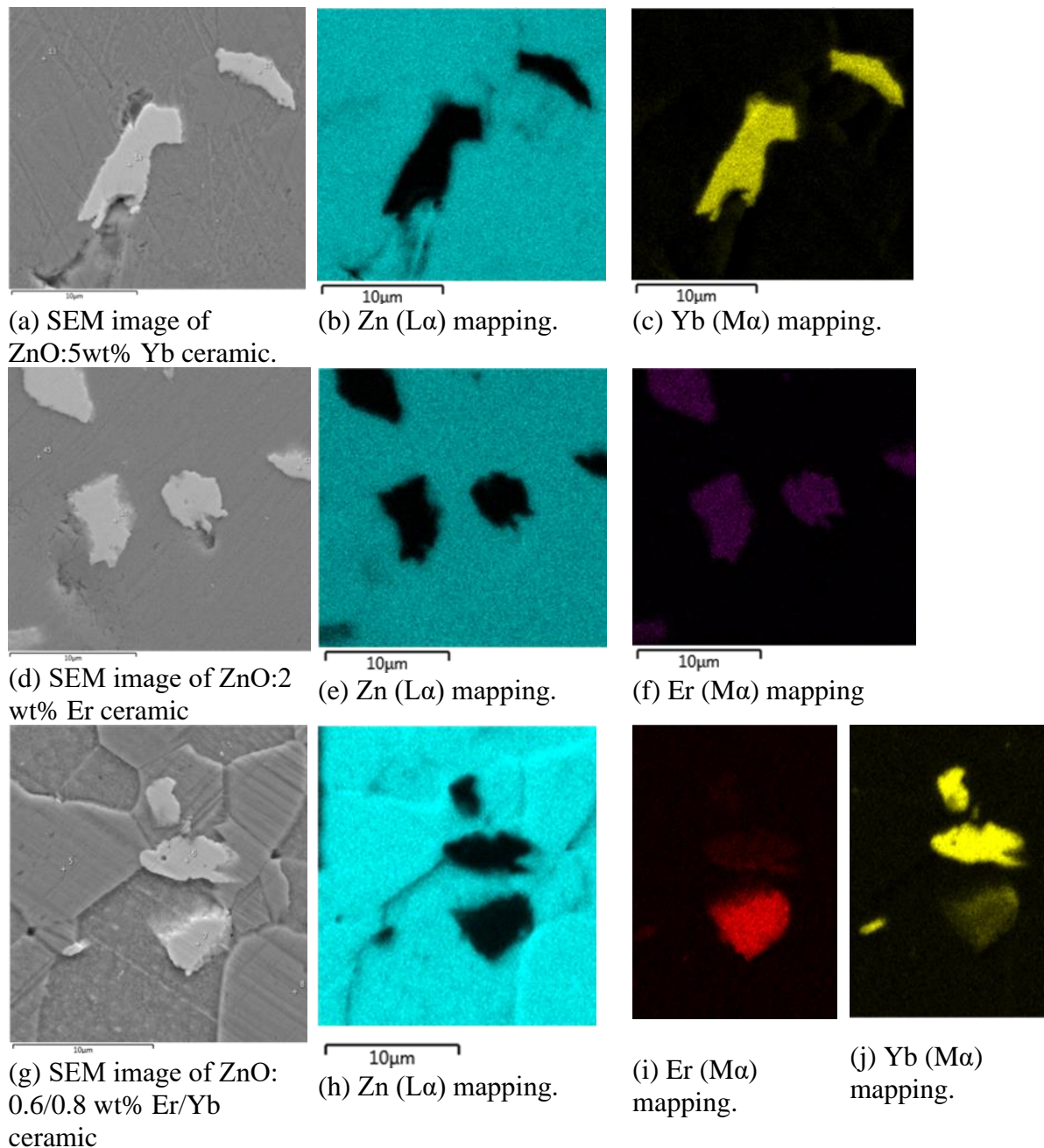
Fig. 1917. (a,d,g) SEM images of the polished and etched surface of the ZnO:RE ceramics; (b,c,e,f,h-j) EDX element mapping of (b,e,h) Zn ( L\alpha ), (c,j) Yb ( M\alpha ) and (f,i) Er ( M\alpha ). (a-c) the ZnO:5Yb ceramic; (d-f) ZnO:2 wt% Er ceramic; (g-j) ZnO:0.6 wt% Er/0.8wt% Yb ceramic.
