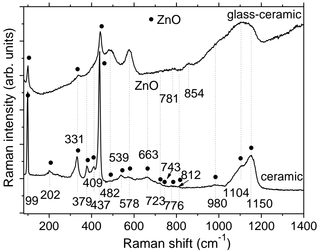
Fig. 25. Raman spectra of the ZnO glass-ceramics doped with 0.1 mol% \text{Yb}_2\text{O}_3 prepared by the heat-treatment at 750 °C for 2 h and of the ZnO:0.2 wt% Yb ceramic.
