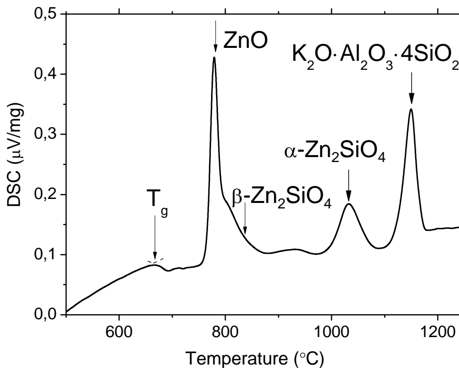
Fig. 5. DSC curve for the glass Zn1 doped with 0.05% CoO.
