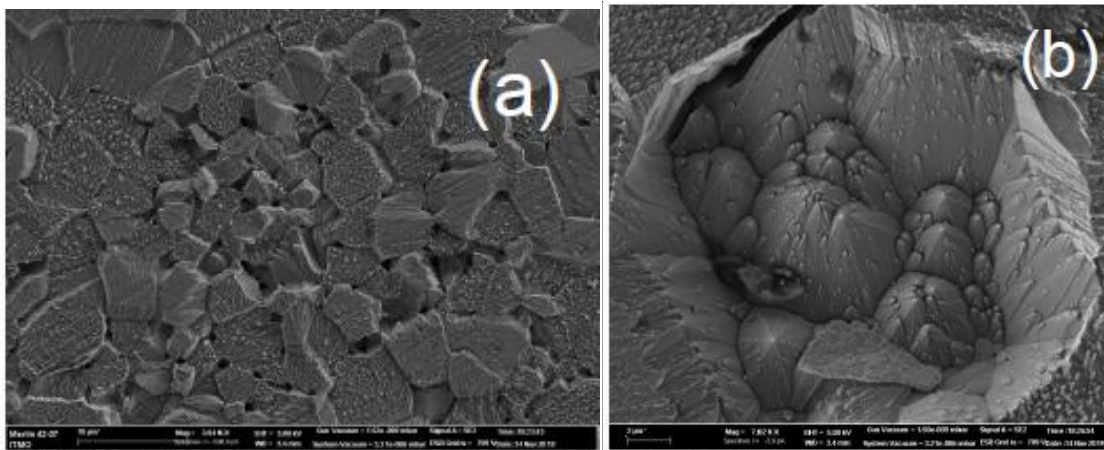
Fig. 1816. SEM images of the polished surface of 0.4 wt% Er-doped ZnO ceramic. The scale bars are (a) 10 \mu\text{m} and (b) 2 \mu\text{m} .
