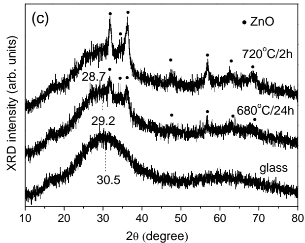
Fig. 3. SAXS curves and XRD patterns for the initial glass Zn1 doped with 0.05% CoO and glass-ceramics: (a) dependences of the SAXS intensity on Q ; (b) dependences of Q \cdot I(Q) on Q ; (c) corresponding XRD patterns. The dashed lines mark the positions of the maxima on the curves. The heat-treatment schedules are shown in figures.
