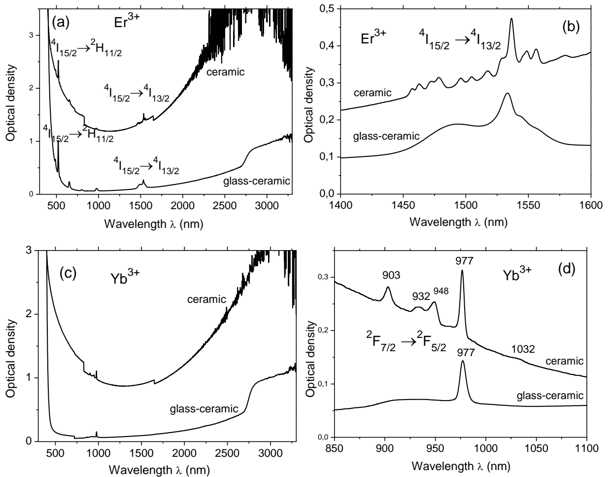
Fig. 27. (a,b) Absorption spectra of the Zn2 glass-ceramics doped with 1.5 mol% \text{Er}_2\text{O}_3 prepared by the heat-treatment at 750 °C for 2 h and the ZnO:3 wt% Er ceramic in the spectral range of 300 – 3300 nm (a); in the spectral range of 1400 – 1600 nm (b). The thickness of the glass-ceramic sample is 1 mm, that of the ceramic sample is 0.5 mm. (c,d) Absorption spectra of the Zn2 glass-ceramics doped with 0.1 mol% \text{Yb}_2\text{O}_3 prepared by the heat-treatment at 680 °C for 48 h and the ZnO:3 wt% Yb ceramic in the spectral range of 300 – 3300 nm (c); in the spectral range of 850 – 1100 nm (d). The thickness of the glass-ceramic sample is 3 mm, that of the ceramic sample is 0.5 mm.
