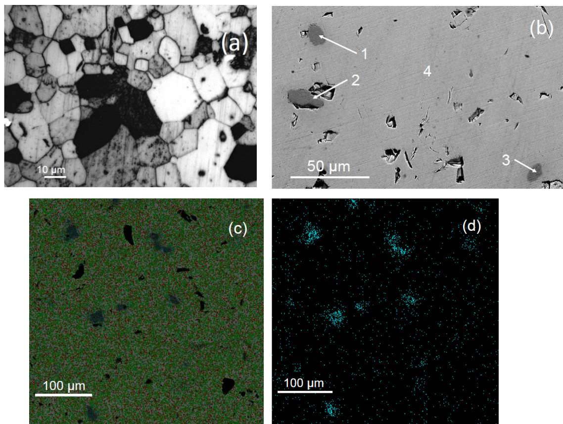
Fig. 2119. (a,b) Micrograph of the etched surface(a) and the backscattered electron image (b) of the ZnO:0.5 wt% Co ceramic; (c,d) EDX Zn, O, and Co element mapping (c) and Co element mapping (d) of the ZnO:1 wt% Co ceramic.
