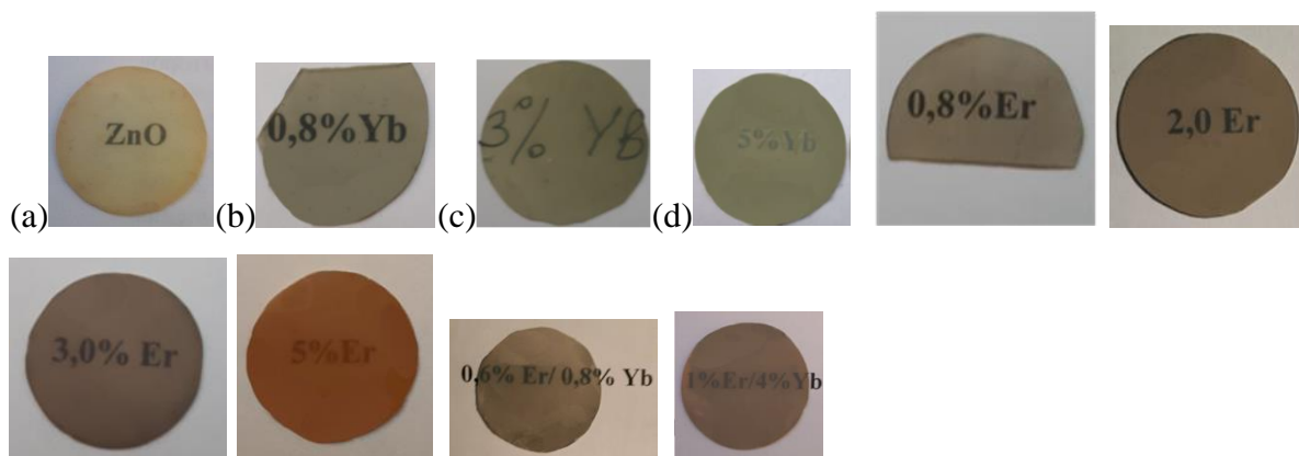
Figure 2. Photographs of (a) undoped and (b-e) ZnO transparent ceramics with different Yb and Er doping levels (indicated by labels, in wt%).
