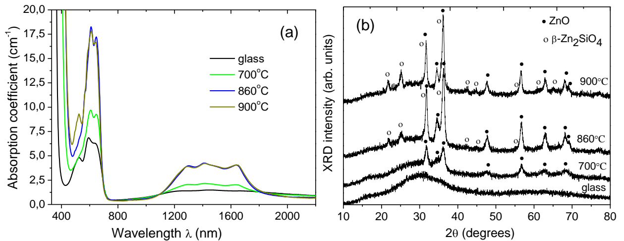
Fig. 7. Absorption spectra (a) and corresponding XRD patterns (b) of the initial and heat-treated glass Zn1 doped with 0.1% CoO. Heat-treatment temperatures are listed in the figure. Heat-treatment time is 2 h.
