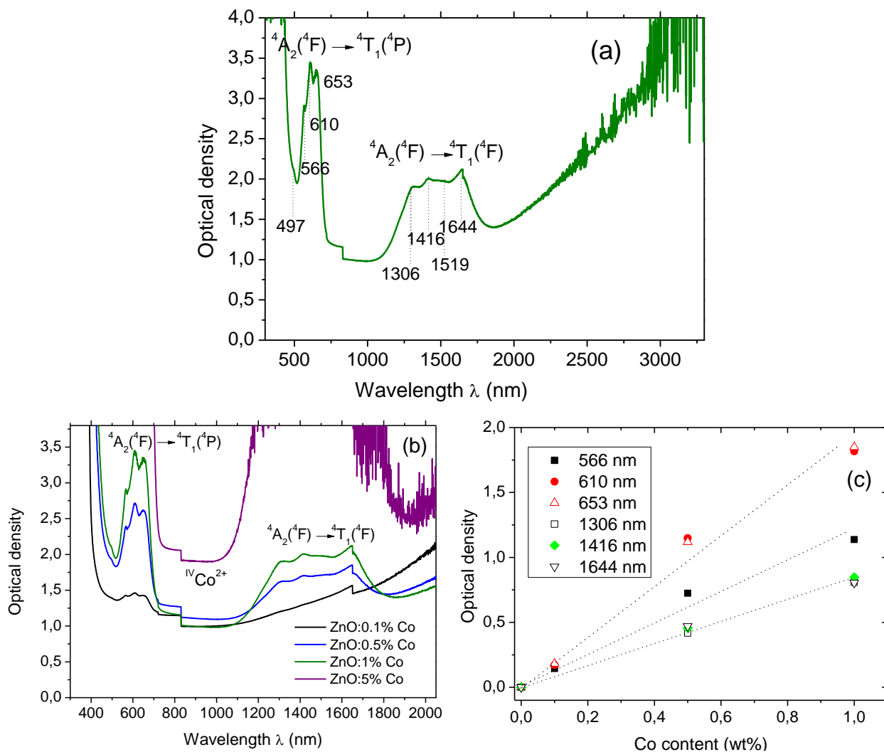
Fig. 2220. Absorption spectrum of ZnO:1 wt% Co ceramic in the spectral range of 300 – 3300 nm (a); absorption spectra of ZnO: Co ceramics doped with 0.1 – 5.0 wt.% Co in the spectral range of 300 – 2050 nm (b); the dependence of the the peak optical density at 566, 610, 653, 1306, 1416, and 1644 nm on the Co content (c). The thickness of the samples is \sim 0.5 mm.
