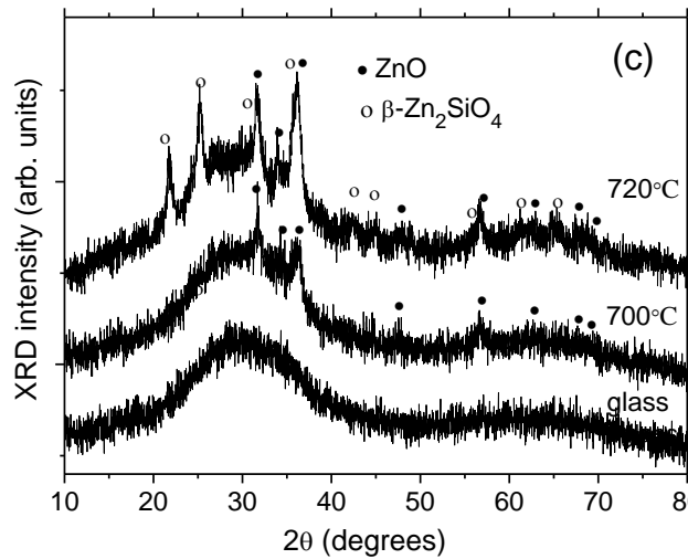
Fig. 9. Absorption spectra (a,b) and corresponding XRD patterns (c) of the initial and heat-treated glass Zn1 doped with 0.1 mol% Cr 2 O 3 . Heat-treatment temperatures are listed in the figure. Heat-treatment time is 2 h.
