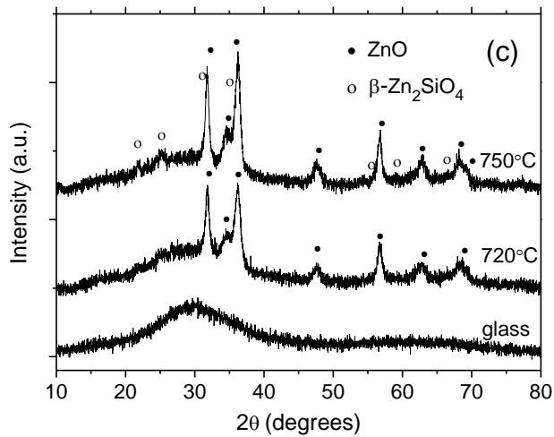
Fig. 8. Absorption spectra (a,b) and corresponding XRD patterns (c) of the initial and heat-treated glass Zn1 doped with 0.2 mol% NiO. Heat-treatment temperatures are listed in the figure. Heat-treatment time is 2 h.
