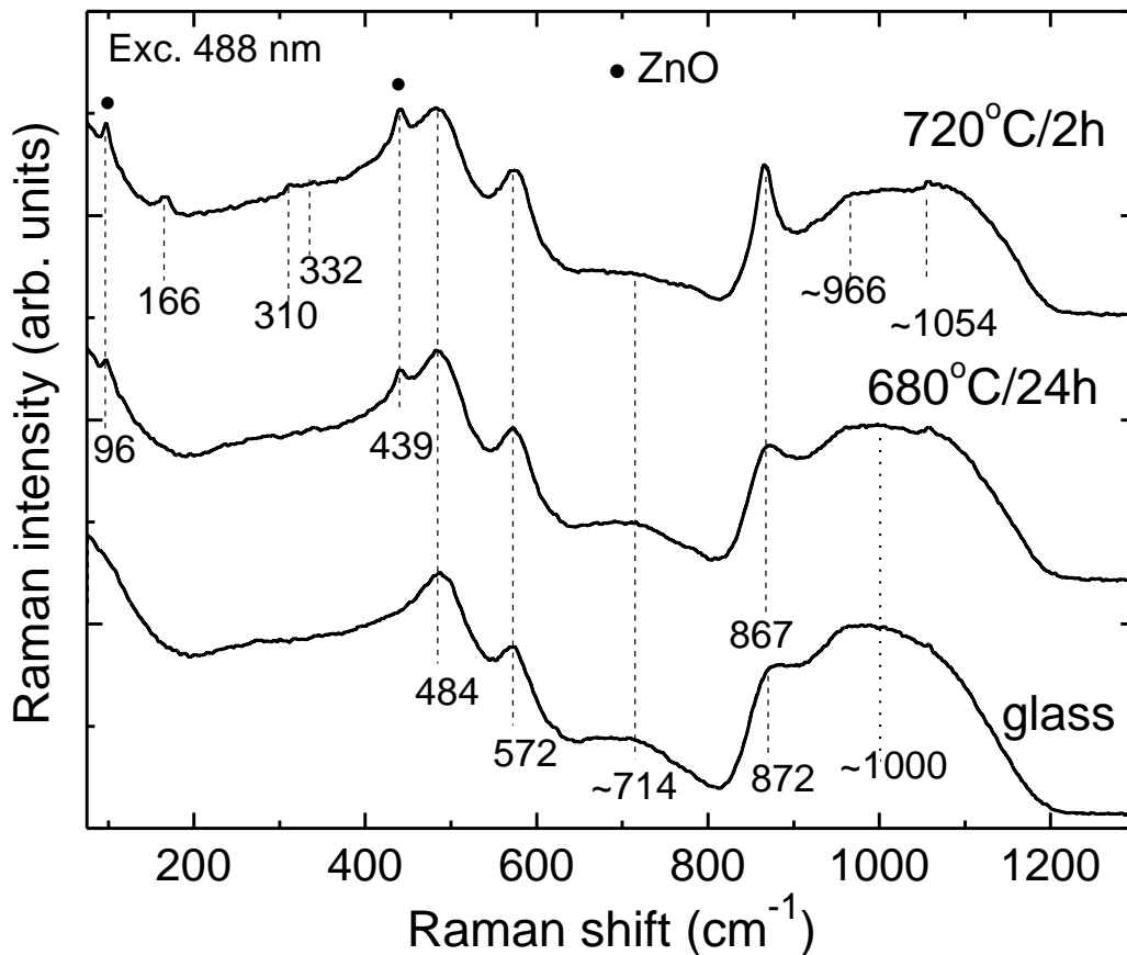
Fig. 4. Raman spectra (a) and XRD patterns (b) for the glass Zn1 doped with 0.05% CoO and glass-ceramics. The heat-treatment schedules are shown in figure.
