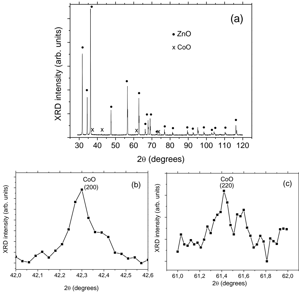
Fig. 2018. (a) XRD pattern of the ZnO: 1 wt% Co ceramic; (b) XRD pattern of ZnO: 1 wt% Co ceramic in the 2\theta range of 42.0 - 42.6^\circ corresponding to the (200) peak of CoO; (c) XRD pattern of ZnO: 1 wt% Co ceramic in the 2\theta range of 61.0 - 62.0^\circ corresponding to the (220) peak of CoO.
