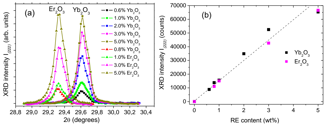
Fig. 1614. (a) XRD patterns of ZnO:RE ceramics with different Er and Yb doping levels in the 2\theta range of 28.9–30.3° corresponding to (222) peaks of Er_2O_3 and Yb_2O_3 ; (b) dependence of the corresponding peak diffraction intensity at 2\theta of 29.33° and 29.63° on the RE content.
