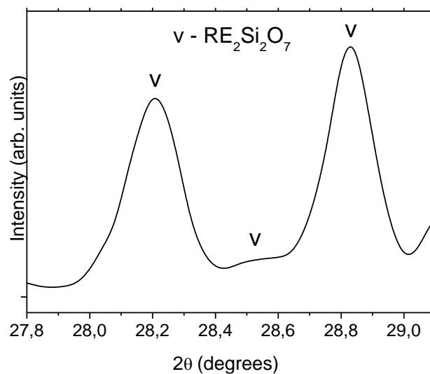
Fig. 1412. The part of XRD pattern of the glass-ceramic doped with 0.1% \text{Er}_2\text{O}_3 and 0.1% \text{Yb}_2\text{O}_3 after heat-treatments at 1300 °C for 2 h recorded in a scanning mode ( 2\theta=27.6\text{--}29.8^\circ ) with 100 s exposure time.
