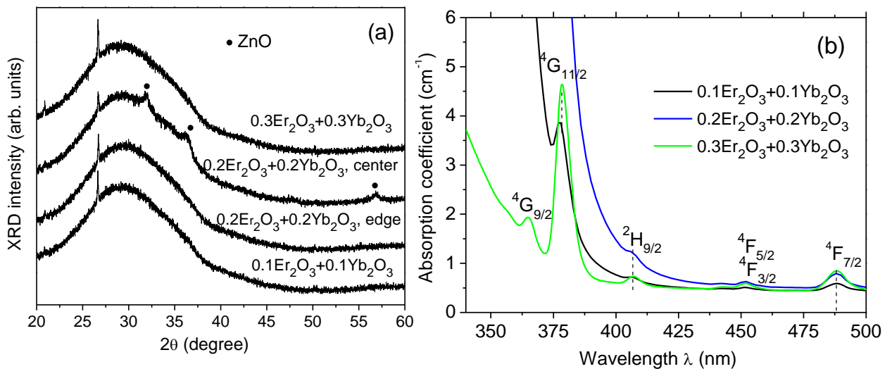
Fig. 1210. XRD patterns (a) and absorption spectra (b) of the initial Zn glasses co-doped with \text{Er}_2\text{O}_3 and \text{Yb}_2\text{O}_3 . The \text{Er}_2\text{O}_3 and \text{Yb}_2\text{O}_3 doping level is indicated in figure.
