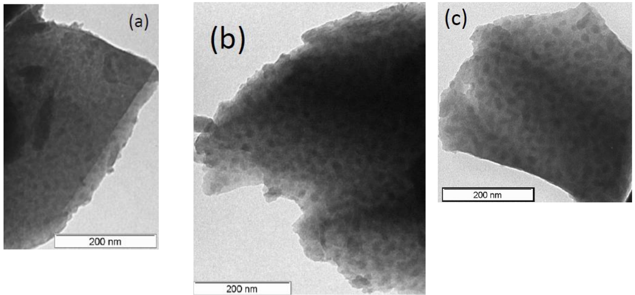
Fig. 119. TEM images of the initial Zn glasses doped with (a) 0.1% \text{Er}_2\text{O}_3 and 0.1% \text{Yb}_2\text{O}_3 ; (b) 0.2% \text{Er}_2\text{O}_3 and 0.2% \text{Yb}_2\text{O}_3 ; (c) 0.3% \text{Er}_2\text{O}_3 and 0.3% \text{Yb}_2\text{O}_3 .
