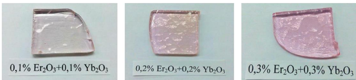
Fig. 10. 8. Images of the initial Zn 2 glasses doped with (a) 0.1% \text{Er}_2\text{O}_3 and 0.1% \text{Yb}_2\text{O}_3 ; (b) 0.2% \text{Er}_2\text{O}_3 and 0.2% \text{Yb}_2\text{O}_3 ; (c) 0.3% \text{Er}_2\text{O}_3 and 0.3% \text{Yb}_2\text{O}_3 .
