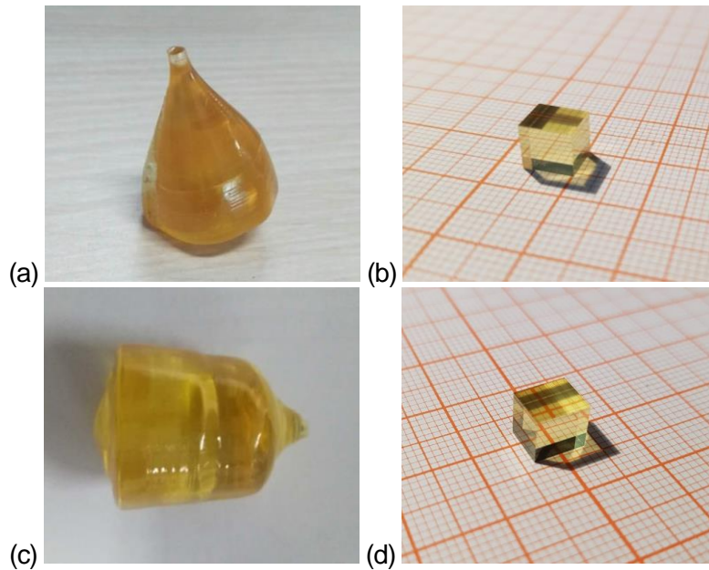
Fig. 1. (a-d) Photographs of the \text{Tm,Ho:Ca(Gd,Lu)AlO}_4 crystals grown by the Czochralski method: (a,c) as-grown crystal boules, (b,d) polished cubic samples oriented along crystallographic axes; (a,b) 5.5 at.% \text{Lu}^{3+} , (c,d) 10.8 at.% \text{Lu}^{3+} (in the crystal). The full chemical formulas are given in Table 1. The growth direction is along the [001] axis.
