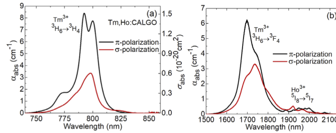
Fig. 2. Polarized absorption spectra of the 4.5 at.% Tm, 0.5 at.% Ho:CALGO crystal: (a) {}^3\text{H}_6 \rightarrow {}^3\text{H}_4 Tm 3+ transition, (b) {}^3\text{H}_6 \rightarrow {}^3\text{F}_4 Tm 3+ and {}^5\text{I}_8 \rightarrow {}^5\text{I}_7 Ho 3+ transitions.
