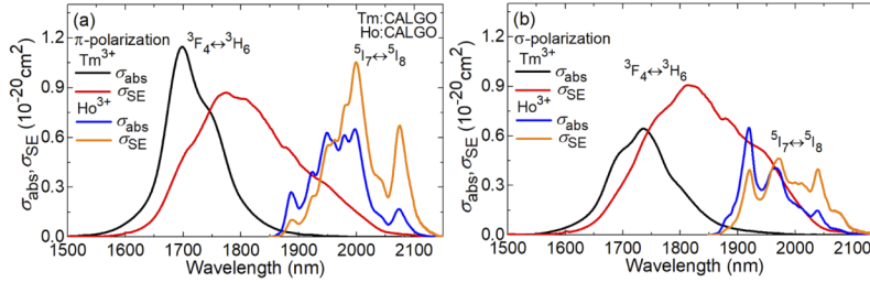
Fig. 4. Absorption, \sigma_{\text{abs}} , and stimulated-emission (SE), \sigma_{\text{SE}} , cross-sections for \text{Tm}^{3+} and \text{Ho}^{3+} ions in CALGO around \sim 2 \mu\text{m} , the light polarization is (a) \pi and (b) \sigma .
