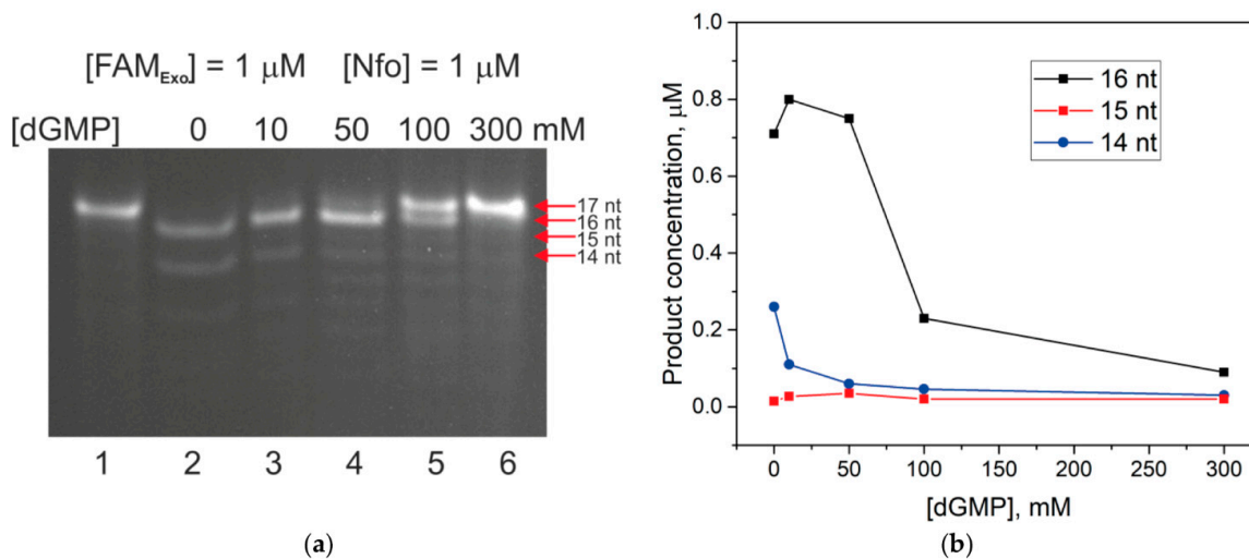
Figure 7. The ratio of the initial DNA substrate to products during the interaction between Nfo and FAM_{Exo} in the presence of 2'-deoxyguanosine monophosphate (a). Amounts of 16- and 15-mer products in the reaction mixture as a function of dGMP concentration (b). [Nfo] = 1.0 \mu M and [FAM_{Exo}] = 1.0 \mu M ; [dGMP] varied from 0 to 300 mM.
