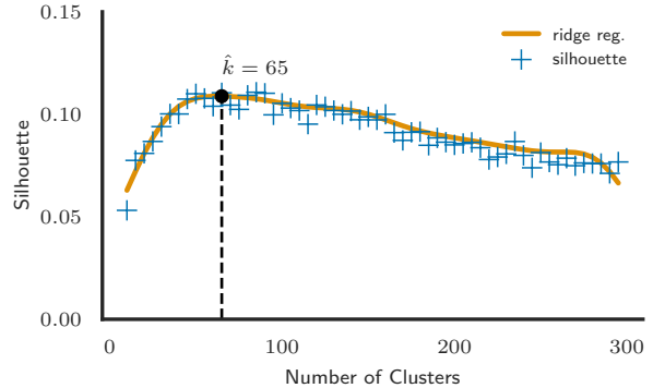
Figure 2: Results of the Elbow Rule on FewRel. Estimated number of relations \hat{k} is equal to 65.
