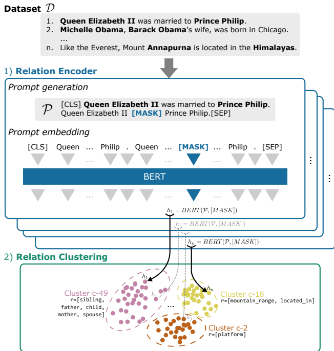
Figure 1: Overview of PromptORE.
