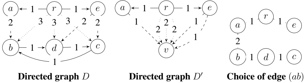
Figure 2: Three stages of unravelling the LIQUID profile B from Table 2 by using Edmonds' algorithm. The directed graph D (left) represents the initial profile. In D' (centre), the nodes b , c and d are contracted into v , as they were in a cycle in D . The arborescence tree (right) is the output where the edge (ab) was chosen to break the tie, and it corresponds to an outcome of MINSUM on B .
