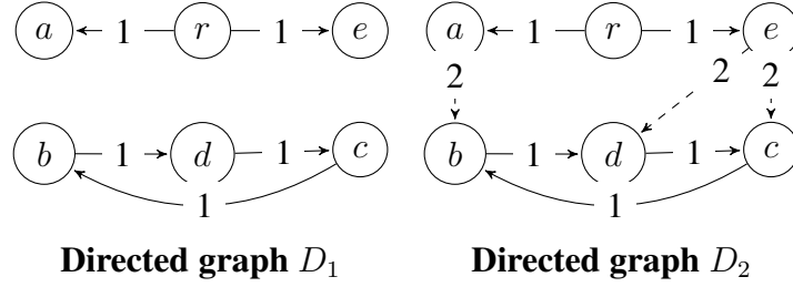
Figure 3: Application of the algorithm in the proof of Theorem 4 to the LIQUID profile \mathbf{B} from Table 2. The directed graph D_1 (left) shows the first iteration of the algorithm for the first preference levels of the agents. As in D_1 there is not a path from r to every other node, the algorithm moves to the second iteration, constructing D_2 (right), which shows the agents' first and second preference levels. Since D_2 is connected, the algorithm terminates.
