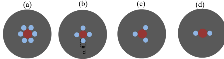
Fig. 3. New concept of fiber entitled D-HNLF in which the initial trench is discretized into either (a) six low- n inclusions (6I), (b) four low- n inclusions (4I), (c) three low- n inclusions (3I) or (d) two low- n inclusions (2I).
