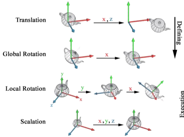
Figure 6. Object transformation order in application code
