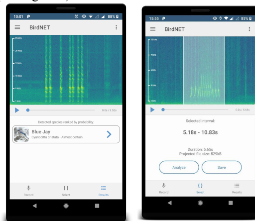
Figure 4. BirdNET Application
