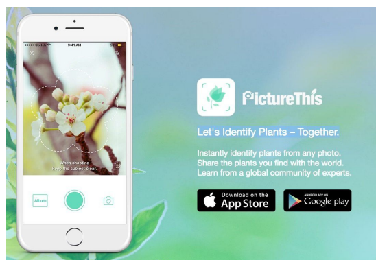
Figure 3. PictureThis Application
