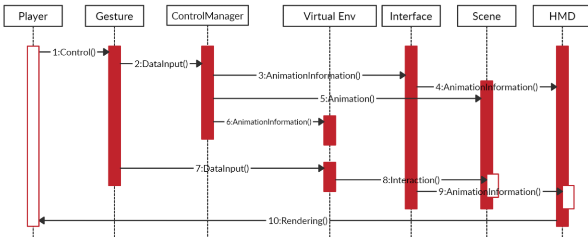
Figure 6 – Sequence diagram
