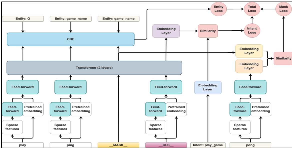
Figure 1. DIET architecture [8].
