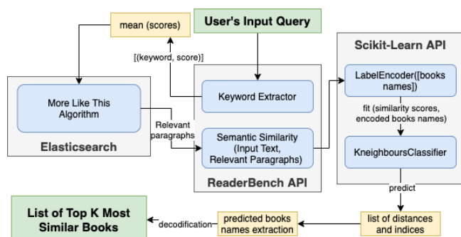
Figure 8. Semantic search algorithm.
