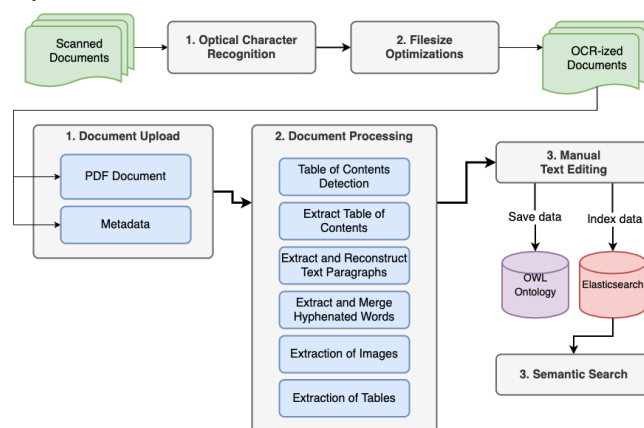
Figure 2. Lib2Life document processing workflow.
