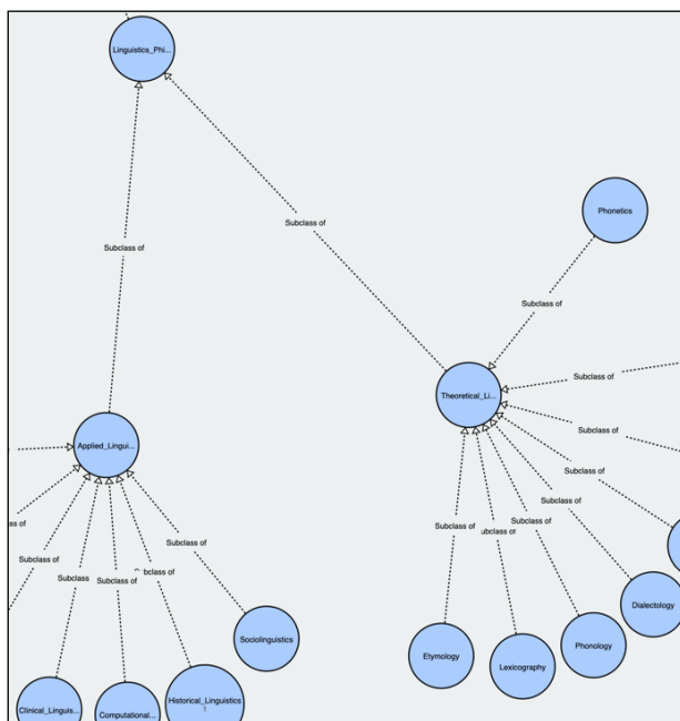
Figure 11. The Lib2Life ontology viewer.
