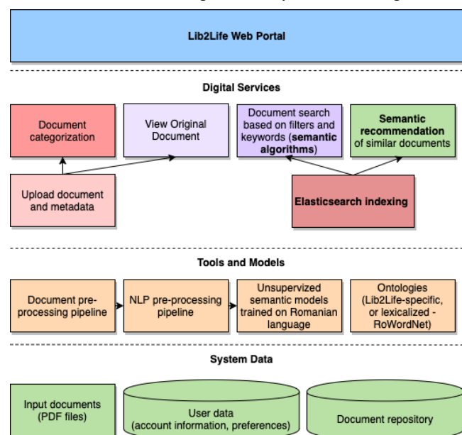
Figure 1. Lib2Life platform architecture.
