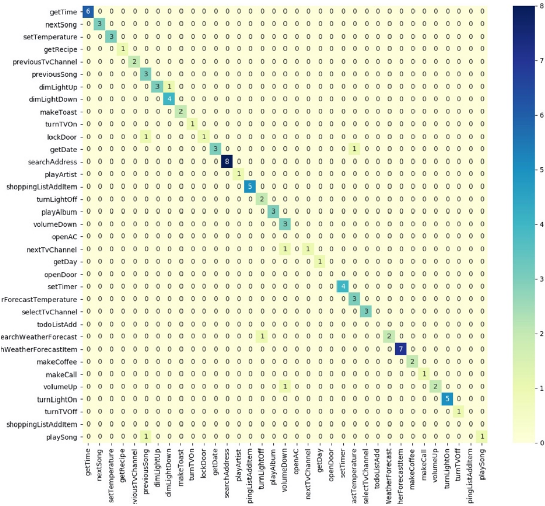
Figure 9. Confusion matrix for the first microworld (home assistant).
