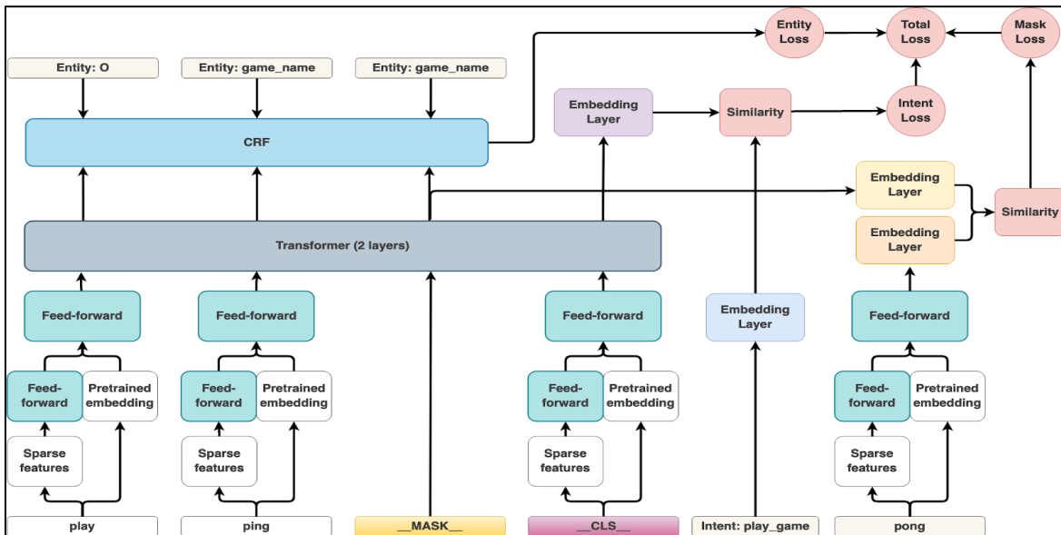
Figure 1. DIET architecture [8].
