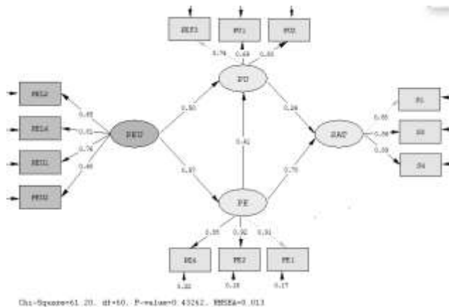
Figure 2. Structural model
