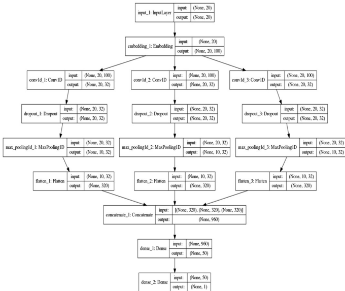
Figure 4. Neural network with 3 CNN channels
