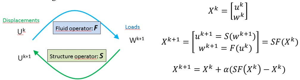
Figure 4: Fluid-structure fixed-point algorithm
