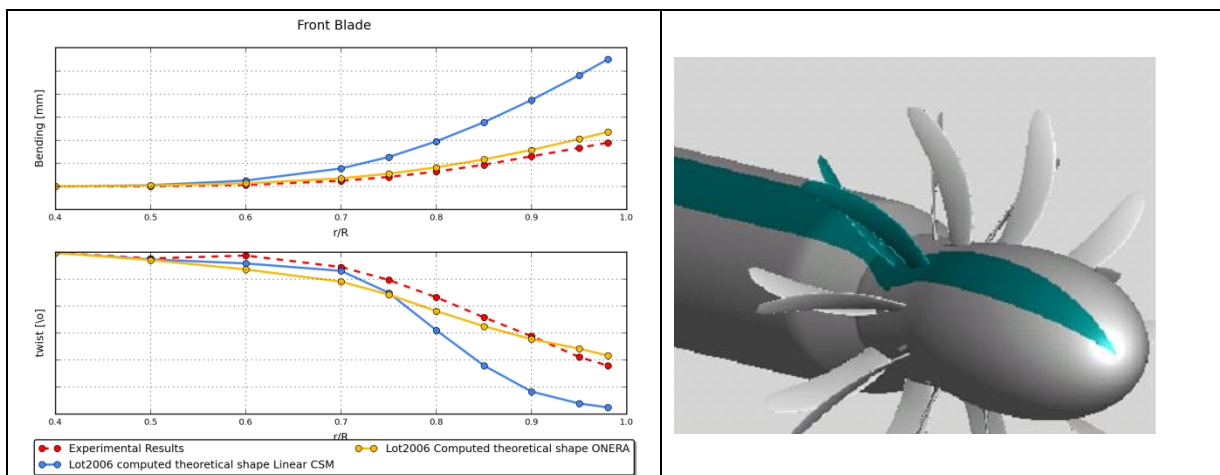
Figure 7: AIXP7 at Z49 rig - CFD-CSM coupling simulation @ cruise conditions M=0.75
