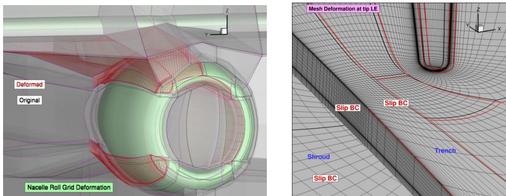
Figure 2: Mesh deformation examples using elastic analogy: oscillating nacelle (a), axial compressor with trench clearance at shroud (b)
