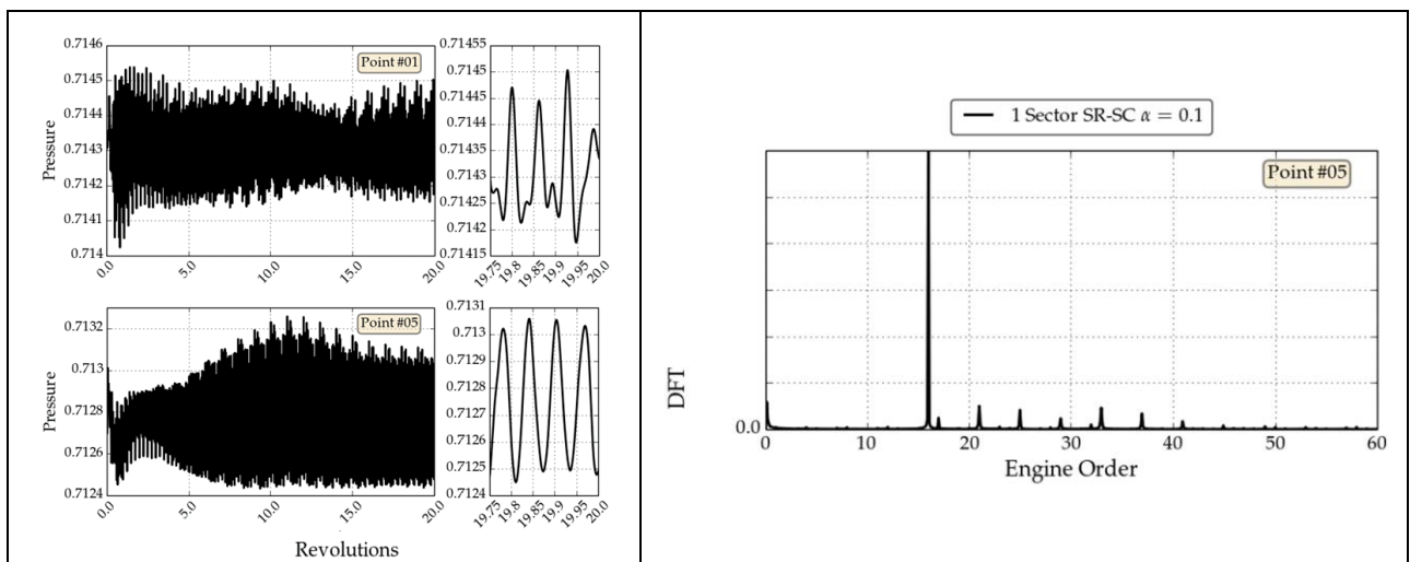
Figure 15: 3D sector model - Pressure sensors history on R1 blade (top left) – in R1 channel (bottom left), Frequency content in R1 channel (right)
