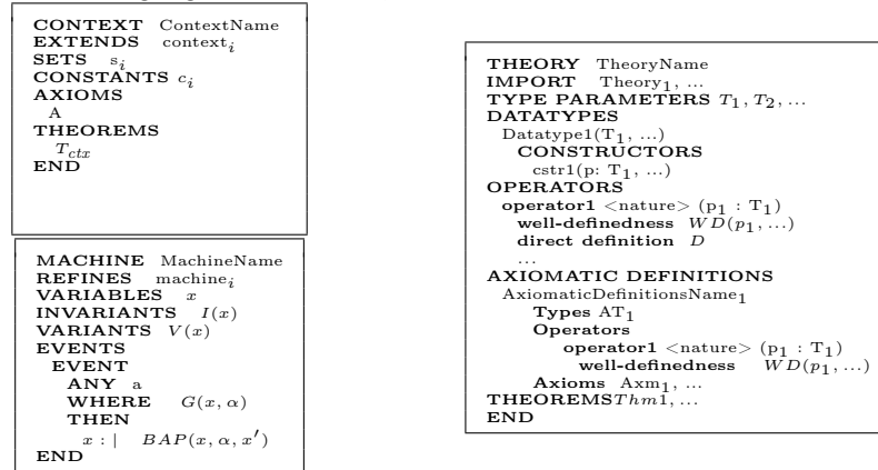
Lst. 1.1: Basic Event-B building blocks: context, machine and theory
