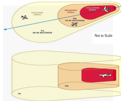
Fig. 1: Protection Volume
