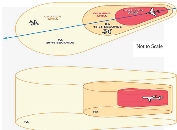
Fig. 1. Protection volume
