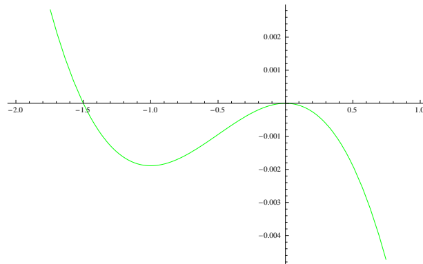
Figure 5: The h-curve for Eq. (30) obtained by the 3^{rd} order approximation.
