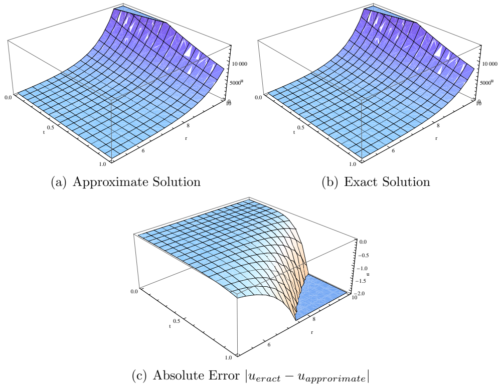
Figure 4: Solution profiles of the equation (21): (a) approximate solution (b) exact solution (c) absolute error |u_{exact} - u_{approximate}| .
