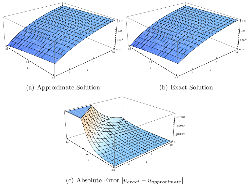
Figure 2: Solution profiles of the equation (12): (a) approximate solution (b) exact solution (c) absolute error |u_{exact} - u_{approximate}| .
