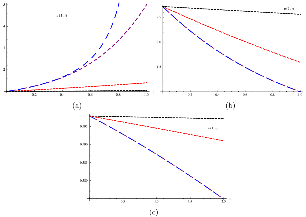
Figure 7: The results obtained by HAM for different values of h for Eqs. (12), (21) and (30) as figure (a), (b) and (c), respectively; black line for h = -0.1 , red line for h = -0.01 , purple line for h = -1 and blue line for exact solution.
