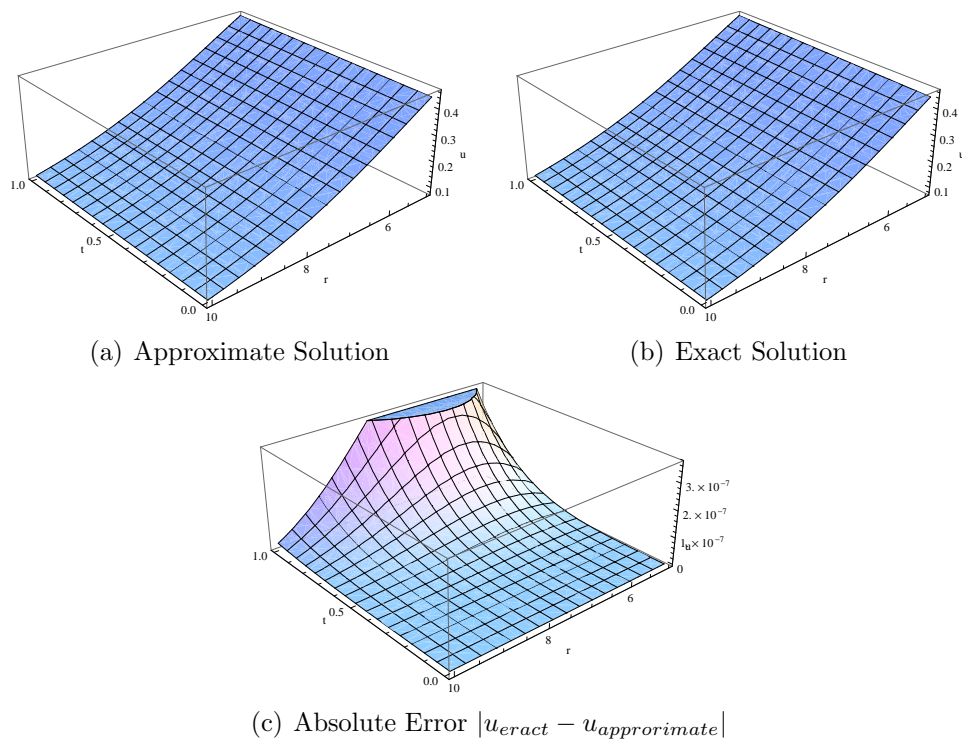
Figure 6: Solution profiles of the equation (30): (a) approximate solution (b) exact solution (c) absolute error |u_{exact} - u_{approximate}| .
