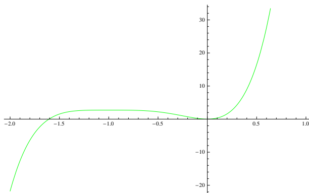
Figure 3: The h-curve for Eq. (21) obtained by the 5 th order approximation.
