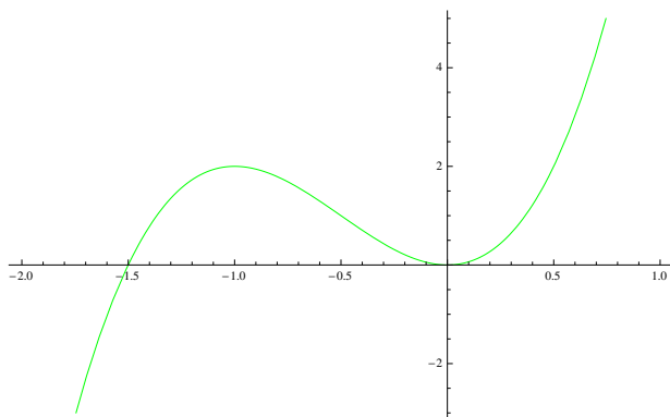
Figure 1: The h-curve for Eq. (12) obtained by the third order approximation.
