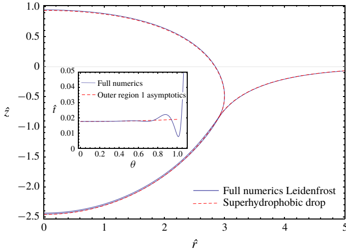
FIGURE 9. (Colour online) Profiles calculated for equal property liquids, \mathcal{R} = 3 and \mathcal{E} = 8.64 \times 10^{-8} . Both the superhydrophobic drop calculation and the numerical simulation of the full problem yield a spherical cap solution of curvature 2/\mathcal{R}_c for the gap geometry, in agreement with (3.2). Note that for finite-sized drop \mathcal{R}_c \neq \mathcal{R} and the neck is positioned at \theta_n = 1.01 .
