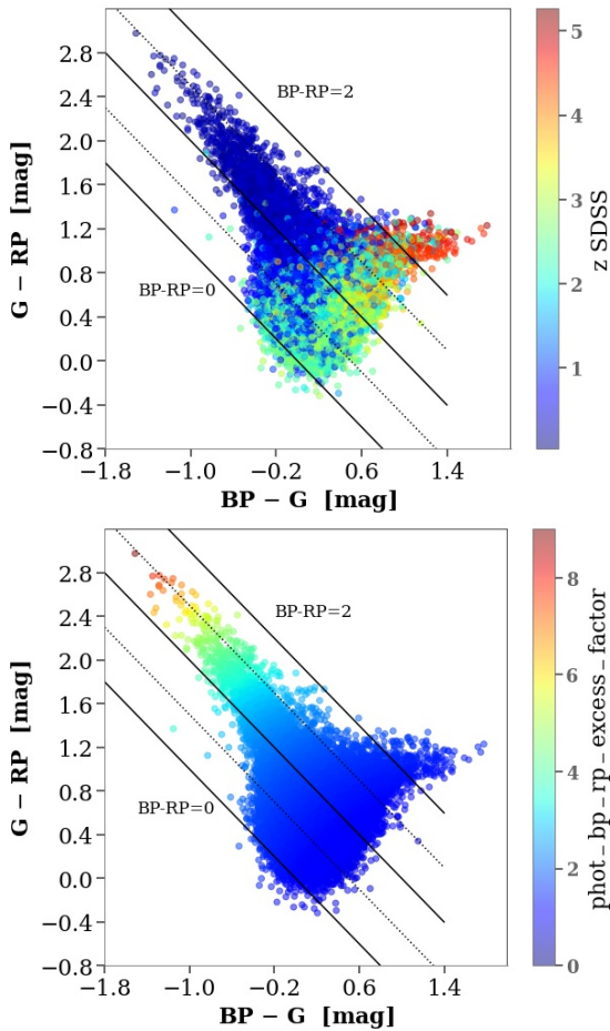
Fig. 31. Colour-colour diagram for the set in Fig. 30 colour-coded by redshift ( top ) and Gaia phot_bp_rp_excess_factor ( bottom ). The straight lines correspond to fixed G_{BP} - G_{RP} colour, with values 2, 1.5, 1, 0.5 and 0.
