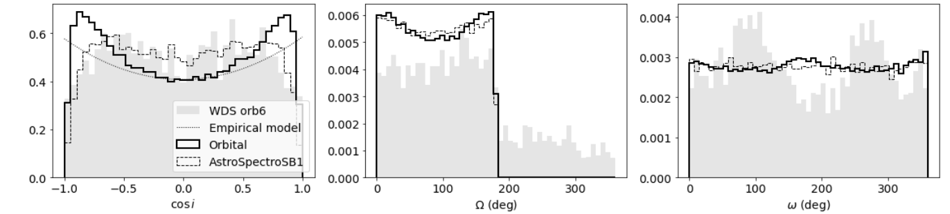
Fig. 11. Normalised distributions of \cos i ( left ), \Omega ( middle ), and \omega ( right ) parameters. Orbital (solid lines, 122989 entries) and AstroSpectroSB1 (dashed lines, 29770 entries) solutions with P < 1000 d are shown. The orb6 solutions from the literature (3405 entries, without filter on period) are shown in grey. Left panel: the dotted line shows the empirical model defined in Sect. 3.2, which was re-scaled on the five central histogram bins. Right panel: we have suppressed the circular solutions with \omega = 0 .
