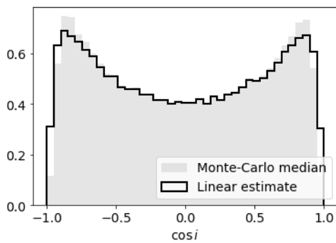
Fig. 13. Normalised distributions of \cos i for non-circular Orbital solutions with P < 1000 d (121 207 entries). The linearised and Monte Carlo estimates are shown as a solid line and a filled grey area, respectively.
