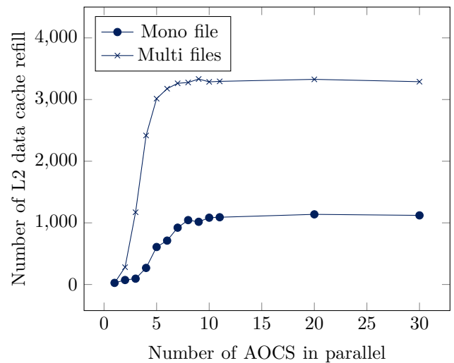
Fig. 5. Measurement of L2 data cache refill in average, comparison of the two processes groups
