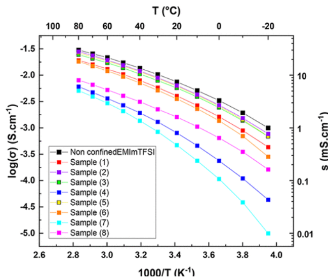
Figure 1. Ionic conductivities for ionogel samples over the range from -20 to 80^\circ C . Ionogel samples were prepared using a variety of processing conditions, including surface modifications and gel calcination, to achieve a variety of porosities and fractal dimensions.
