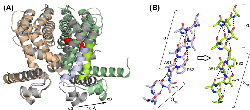
Fig. 2. Comparison of the ligand-bound and ligand-free SCO3201 structures. (A) Superposition of liganded (protein chains shown as beige and green ribbons) and free SCO3201 (dimer AB, grey ribbons). The outward movement of one of the HTH motifs by 10 Å, which coincides with ligand binding to the same protein chain, is indicated by an arrow. The portion of the hinge helix that undergoes substantial conformational changes (bright green and blue in the respective structures) is shown in more detail in panel (B). (B) Conformational changes within the composite hinge helix upon ligand binding. The N-terminal 3_{10} -segment is extended by two residues previously part of the \alpha -helical region (Ala81 and Pro82), leading to stretching and straightening of the hinge helix. All side-chain atoms beyond C_{\beta} have been removed to improve clarity, except those of Pro82. Hydrogen bonds are shown as dashed lines.
