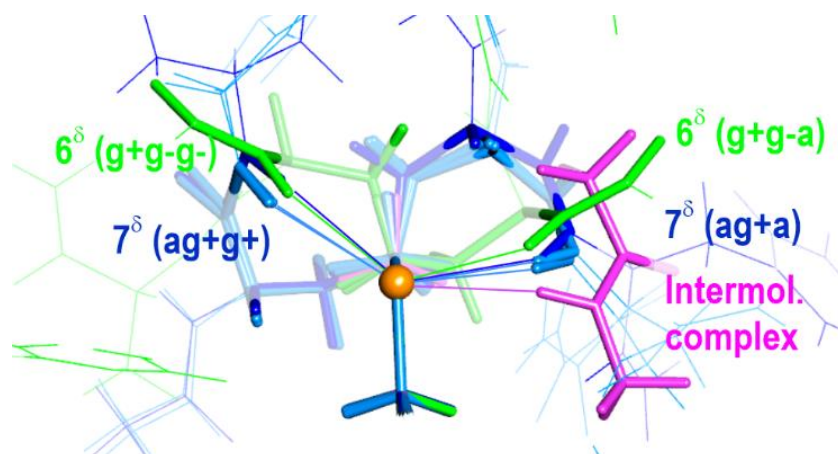
Figure 6. Comparison of the \text{NH} \cdots \text{Se} approaches of the relevant conformations ( 5\text{-}7_{g^+/g^-}^{\delta} light blue, 5\text{-}7^{\delta}/5_a\text{-}\pi dark blue and 6^{\delta}\text{-}\pi_{g^+}\text{-}10 green) of the Ac-Sem-Phe- \text{NH}_2 compound, as found at the DFT-D level of theory. The terminal part of all the Sem side-chains was overlaid (Se atom in dark yellow), allowing to distinguish the effect of the \chi_3 dihedral orientation (side-chain dihedrals between parentheses). For the sake of clarity, front atoms were omitted and background atoms shaded. For reference, the structure of the \text{MAA} \cdots \text{S-SeMe}_2 intermolecular complex was also added. The same figure for the Ac-Met-Phe- \text{NH}_2 compound, provided as Figure S1 in the Supplementary Material, illustrates the similarities between the two species.
