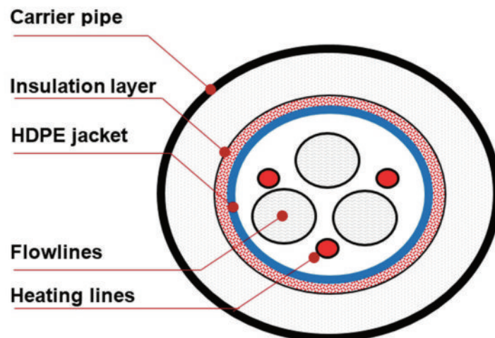
Figure 8. Flowline bundle configuration (adapted from Bai et al. [72]).
