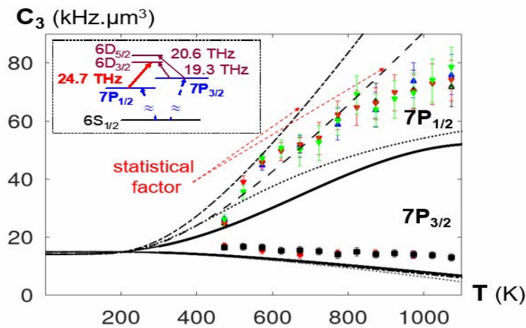
Figure 1: C_3(T) as extracted from atomic spectroscopy (points) on the Cs transitions 6S_{1/2} - 7P_{1/2} and 6S_{1/2} - 7P_{3/2} (see inset), along with various predictions (lines) derived assuming various models for the sapphire permittivity \epsilon(\omega) . The dashed [8] and dashed-dotted [9] lines use sapphire permittivity as determined solely at room temperature, with C_3(T) only governed by a thermal statistics factor; the dotted line [4] and the thick line -our measurements at CEMHTI- involve a temperature-dependence for sapphire permittivity.
