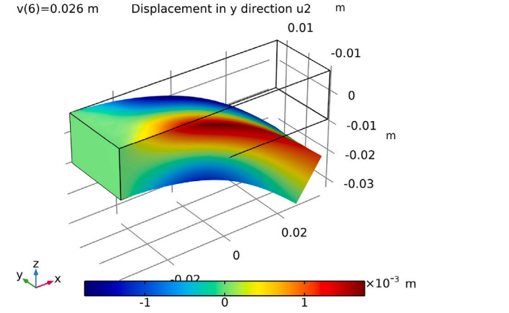
Fig. 5. The shear test on the left is imposed by displacement boundary conditions with colors indicating the amount of deformation energy density by curvature of the embedded fibers. The bending test on the right was conducted with a surface force dead load in z direction. The colors indicate the displacement in y direction, showing the in-plane deformation of the pantographic sheets. (For interpretation of the references to color in this figure legend, the reader is referred to the web version of this article.)
