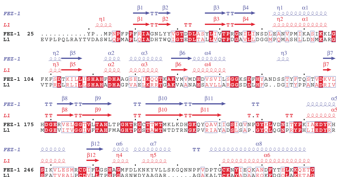
Figure 2. Sequence alignment and secondary structure assignment for FEZ-1 and L1 \beta -lactamases. Residues that are conserved or similar in the two sequences are shown as red and white boxes, respectively. The Figure was made using ESPript. 29
