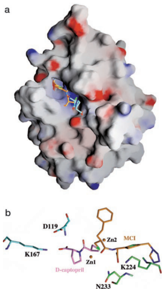
FIG. 3. Two inhibitors in the active site cleft. a , GRASP representation (52) of BlaB complexed with both D-captopril (carbons colored in sky blue) and the mercaptopropionate inhibitor (carbons colored in orange) from the IMP-1 complex (30) after structural superposition of the BlaB and IMP-1 structures. Both molecules intercalate their sulfur atoms between the two zinc atoms of the active site but are localized in different areas of the active site cavity. b , close-up view of the two inhibitors showing strong interactions between the two inhibitors and BlaB.
