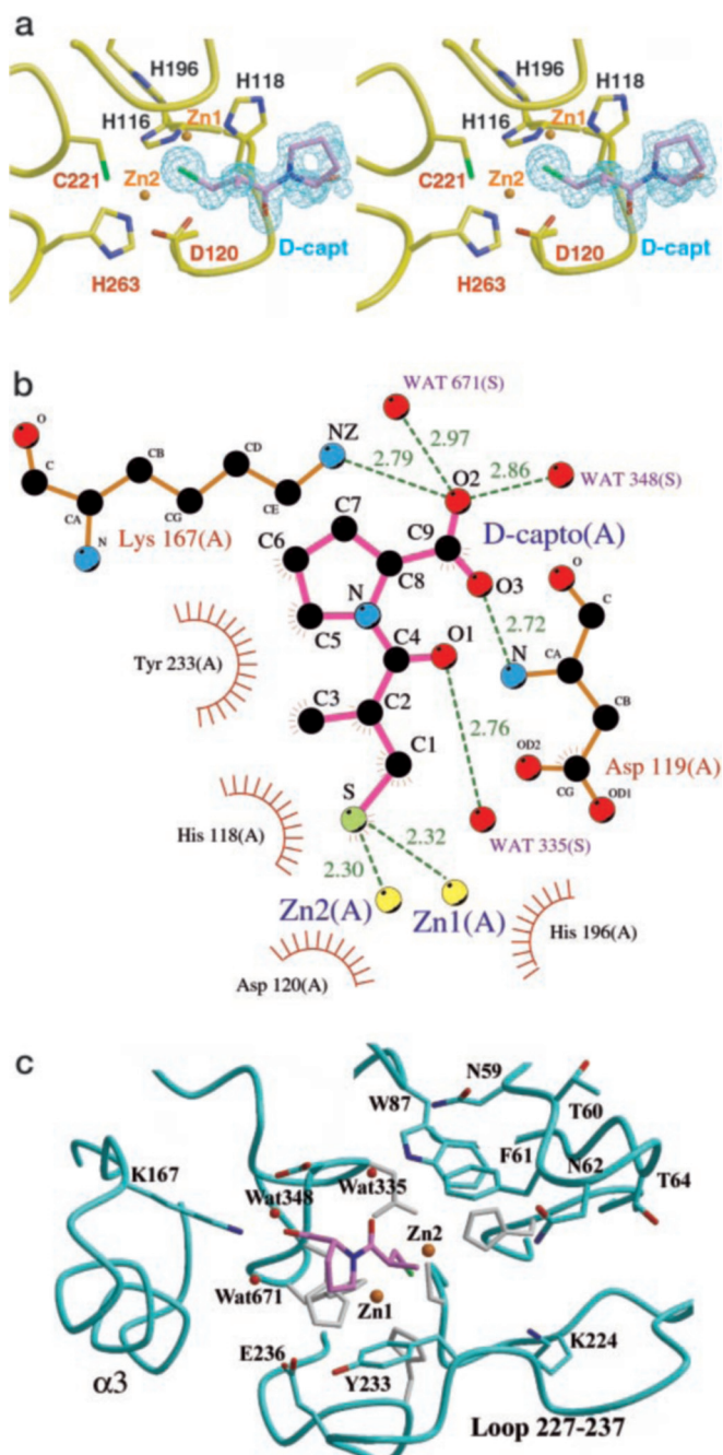
FIG. 2. Coordination of D-captopril by BlaB. a, stereoview of the active site of BlaB in complex with D-captopril. The calculated F_o - F_c map at 1.5 \sigma shows the presence of the inhibitor. The inhibitor atoms were not included in the phase calculation. The residues labeled in black belong to the His site, and those in red belong to the Cys site. Zinc ions are represented as brown spheres. The figure was produced using BOBSCRIPT (54). b, protein-ligand interactions between BlaB and D-captopril depicted in monomer A using LIGPLOT (55). In the schematic drawing, strong interactions are shown as dashed green lines. Ligand and protein hydrophobic contacts are represented as curved red combs. c, active site cleft of BlaB. Zinc ions and water molecules are represented in brown and red spheres, respectively. D-Captopril is displayed in sticks (carbon, nitrogen, and sulfur atoms colored in violet, blue, and green, respectively). Amino acid residues cited in the text under "Structural Comparisons" are labeled, and \text{Zn}^{2+} ligands are colored in gray.
