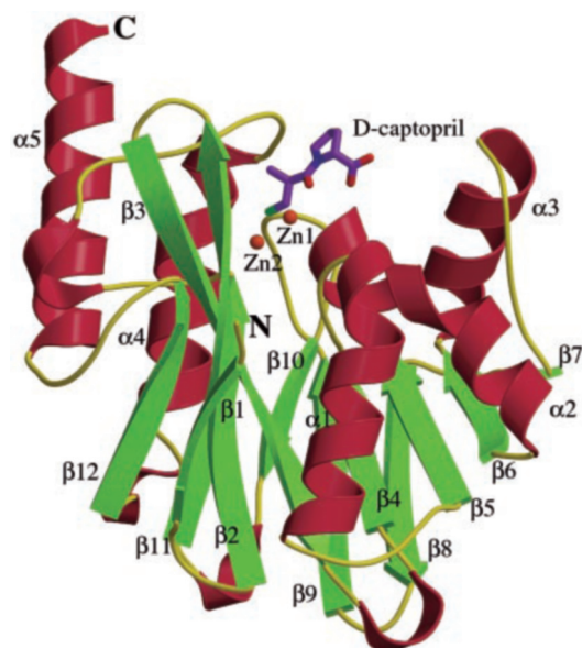
FIG. 1. Structure of BlaB in complex with D-captopril. Three-dimensional structure of BlaB from C. meningosepticum in complex with D-captopril. \alpha -Helices, \beta -Strands, and loops are shown in red, green, and yellow, respectively. \text{Zn}^{2+} ions are represented as dark orange spheres. The N and C termini are labeled. The figure was produced using MOLSCRIPT (53).
