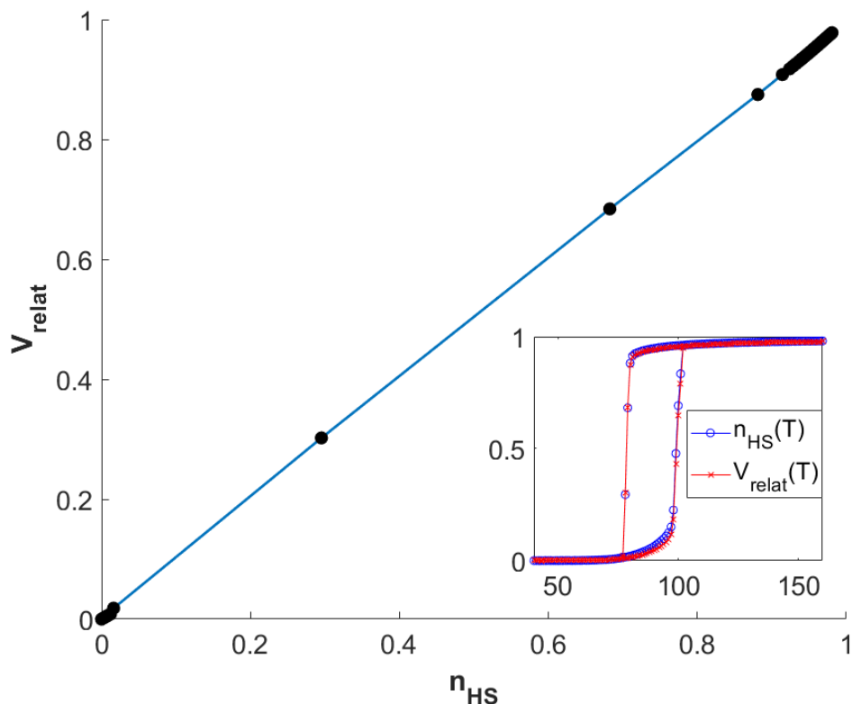
Figure 5 – Elastic variations of the lattice V_{\text{relat}} as a function of electronic variations n_{\text{HS}} during hysteresis loop presented for the case of the cooling branch for A_{1n} = 3\,000 for illustration. The same results are found for the heating branch, or for others elastic constant values. Insert : The two considered variations V_{\text{relat}} and n_{\text{HS}} as a function of T .
