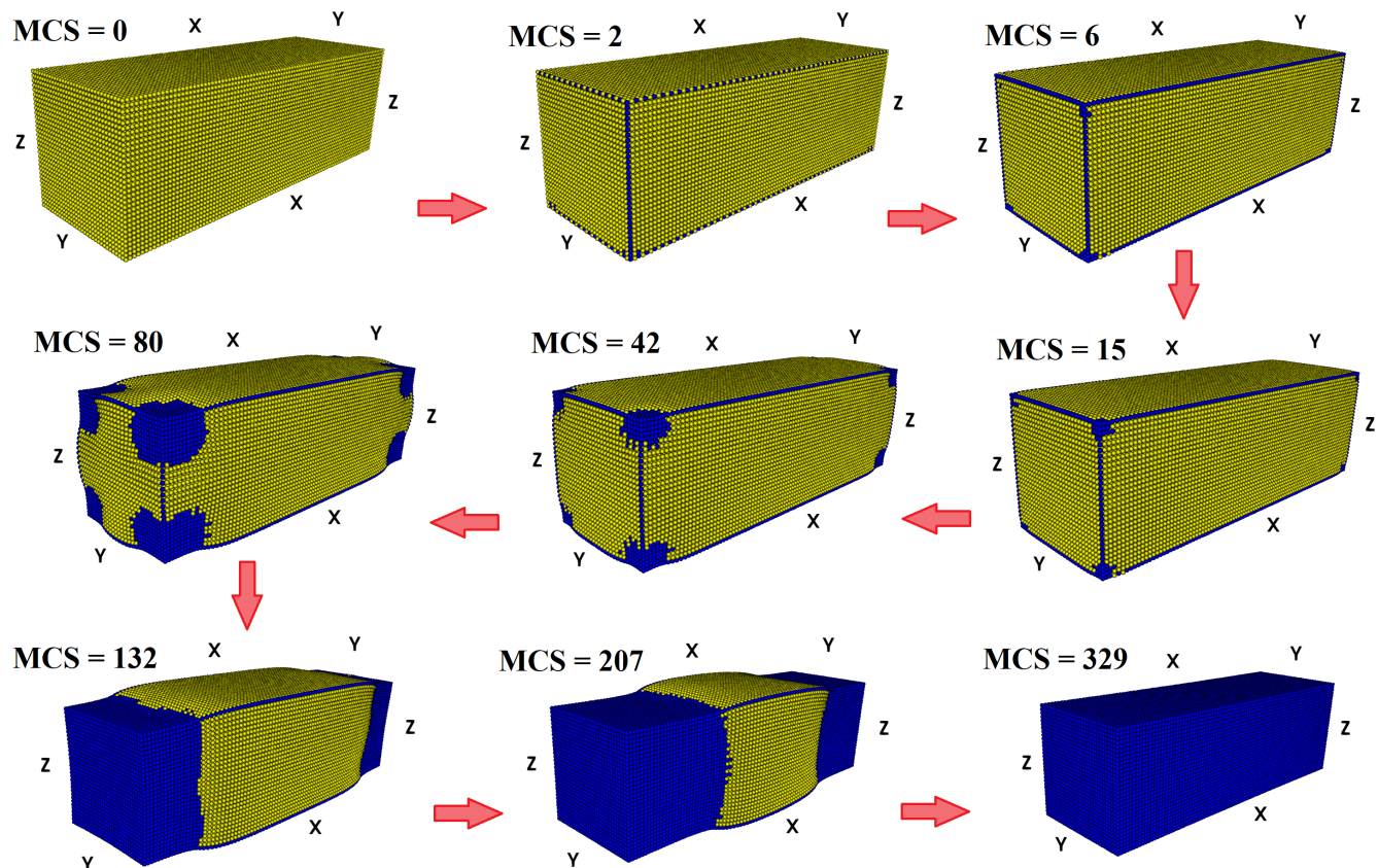
Figure 13 – Snapshots showing the spatiotemporal configurations of the lattice during the relaxation process at T = 1K from an initial HS phase for a large 1n elastic constant value A_{1n} = 7\,000 . Yellow (blue) spheres represent HS (LS) sites.
