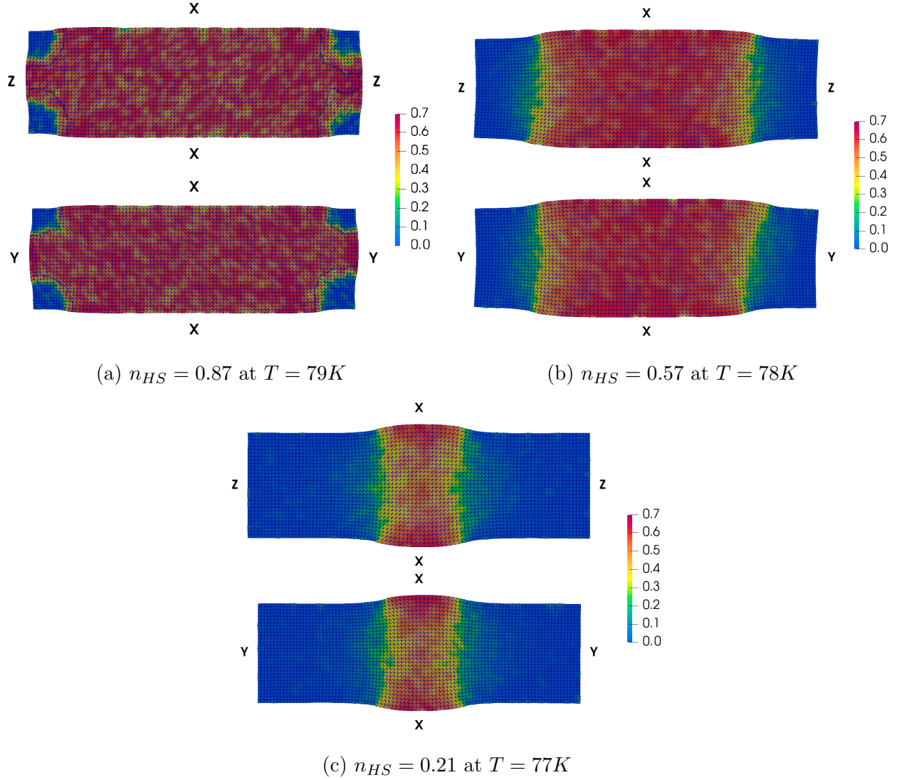
Figure 9 – Sectional view in the planes (xOz) and (xOy) : (a) at N_y (top) and N_z (bottom), and at \frac{N_y}{2} (top) and \frac{N_z}{2} (bottom) for (b) and (c), of the spatial distribution of the divergence of the displacement field corresponding to snapshots of Figure 8.
