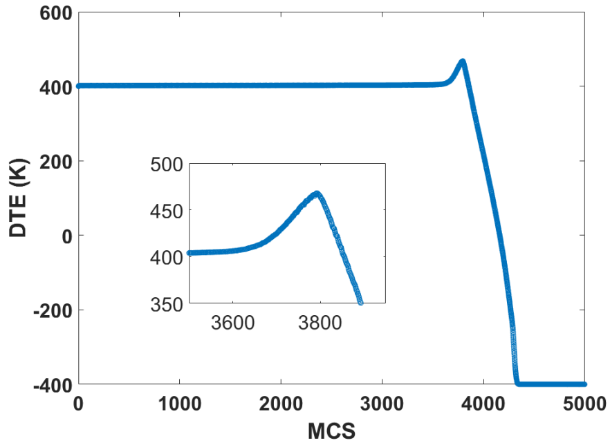
(b) Time-dependence of the DTE. Insert : zoom around the energy barrier of the DTE curve.
