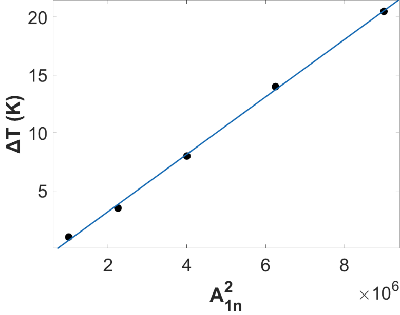
Figure 3 – Hysteresis width \Delta T as a function of the square of the elastic constant values A_{1n} above the critical threshold A_{1n}^C showing a linear behaviour. We take the values of A_{1n} \geq 1\,000\text{ K.nm}^{-2} which are more easily measurable. In blue, we plot a linear regression with 95% confidence bounds.
