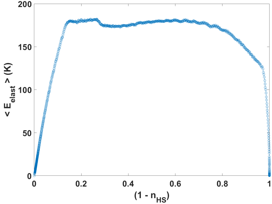
(a) LS fraction dependence of the elastic energy density showing a non-monotonous behavior along the relaxation process. See text for more explanations.
