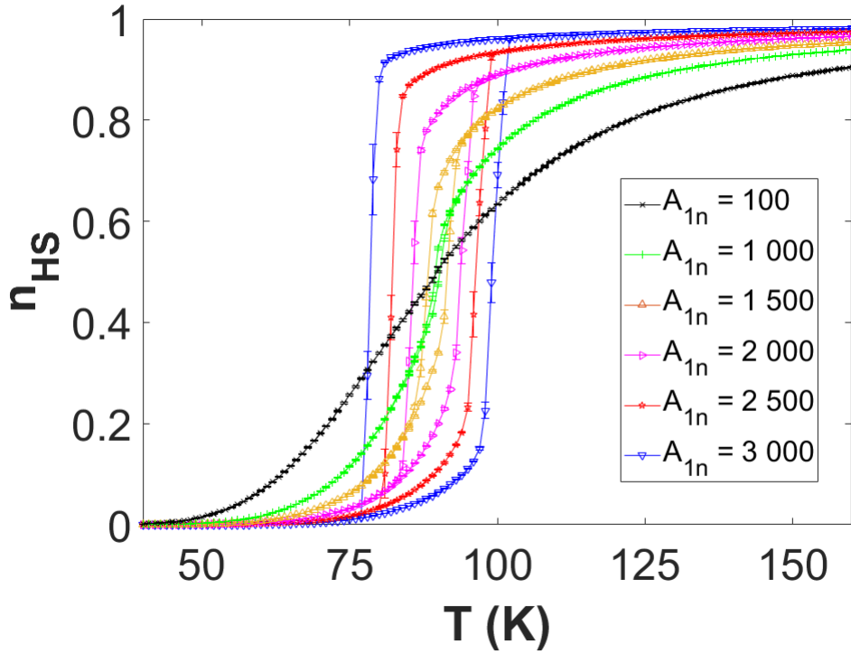
Figure 2 – Thermal dependence of the HS fraction n_{HS} for different values of elastic constants A_{1n} with error bars representing the standard deviation on the average n_{HS} for each temperature for the simulation cell size (96 \times 32 \times 32) . Remark: each presented point has an error bar; however, the latter are visible only near the HS-LS transition, above and below the size of the error bars is smaller than the size of the points.
