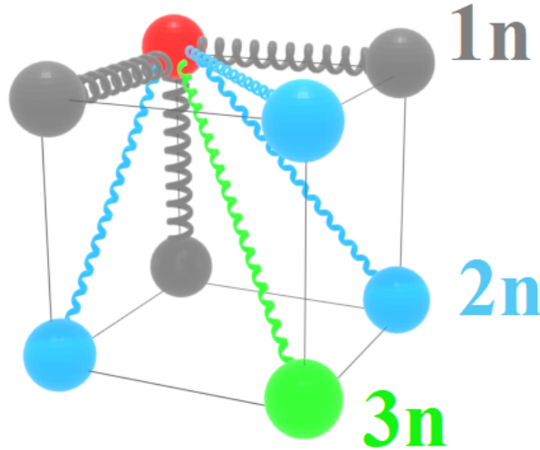
Figure 1 – Schematic view of the 3D elastic network within an elementary simulation cell for a test site represented in red, connected to its neighbours by springs represented in grey for the nearest-neighbours ( 1n ), in blue for the next-nearest neighbours ( 2n ) and in green for the next-next-nearest neighbours ( 3n ). The 1n neighbours are located along the edges of the cube, the 2n neighbours are located along the diagonals of the faces and the 3n neighbours are located along the long diagonals of the elementary cell.
