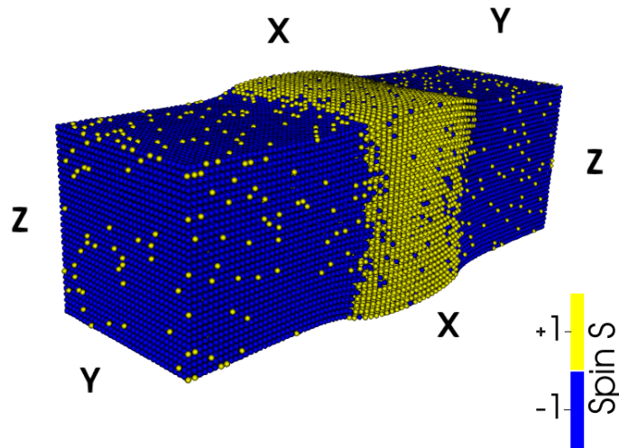
(c) n_{HS} = 0.21 at T = 77K
