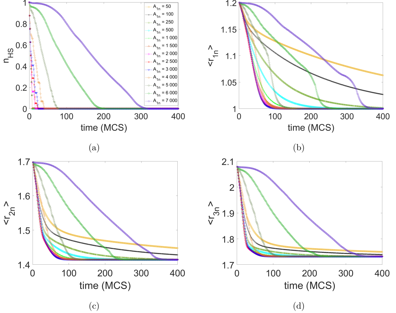
Figure 11 – Time-dependence of the HS fraction (a) and average 1n (b), 2n (c) and 3n (d) lattice parameters along the relaxation from HS to LS of a lattice initially prepared in the HS state at low temperature ( T = 1K ), for various elastic constant, A_{1n} , values. Remark the significant increase of the lifetime of the metastable state with respect to A_{1n} .
