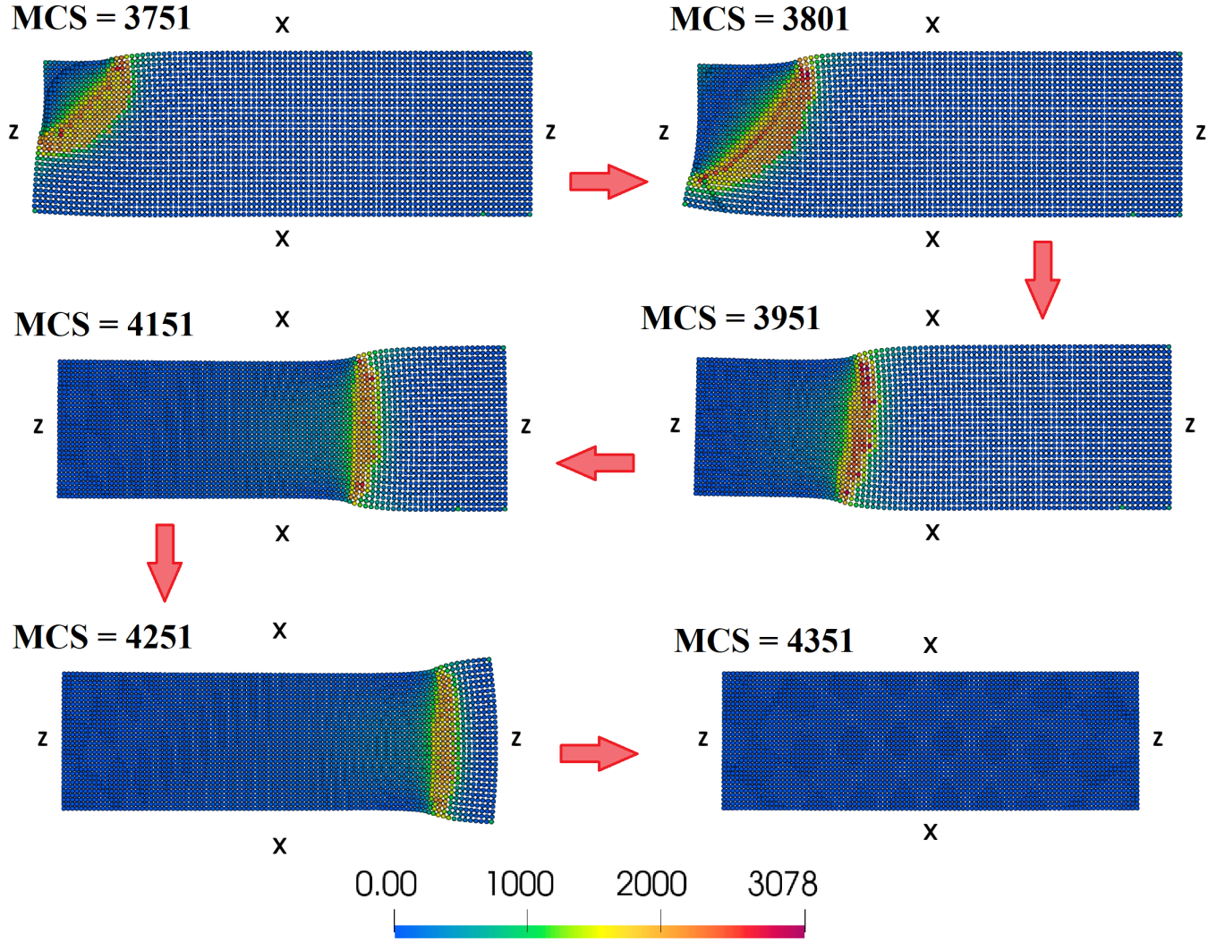
Figure 18 – Sectional view in the plane (xOz) at \frac{N_y}{2} showing the spatial distribution of the local elastic energy field during the relaxation process at T = 10K from an initial HS phase for a large value A_{1n} = 8\,000 .
