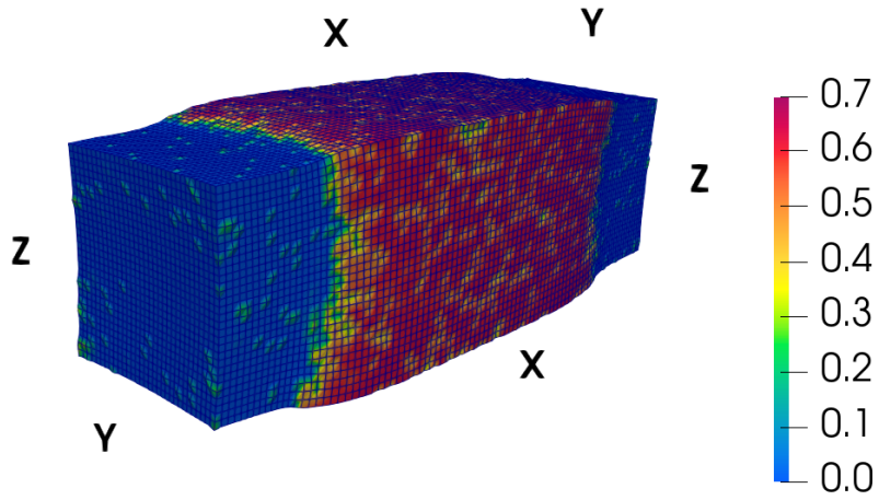
(b) n_{HS} = 0.57 at T = 78K
