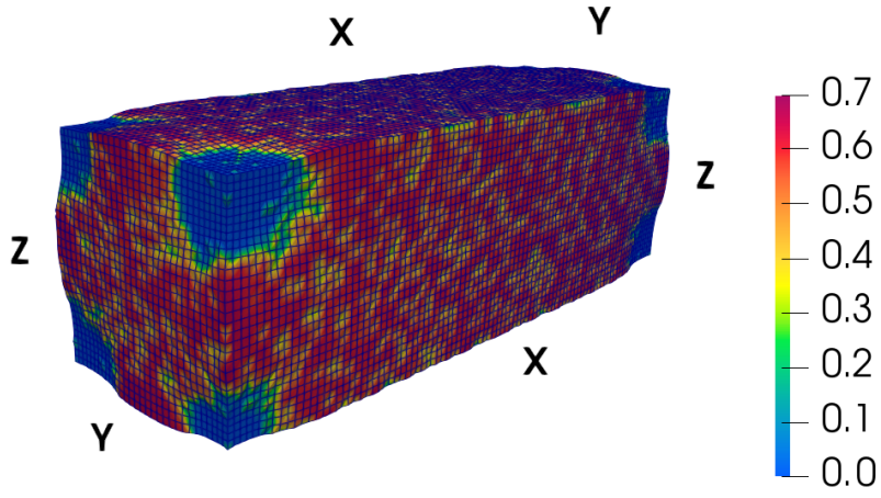
(a) n_{HS} = 0.87 at T = 79K
