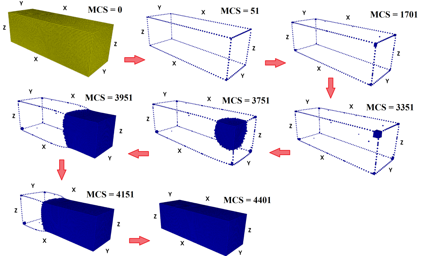
Figure 14 – Specific views of the snapshots showing the spatiotemporal configurations of the lattice during the relaxation process at T = 10K from an initial HS phase for a large value A_{1n} = 8\,000 , with only the LS spins visible during the transition. Yellow (blue) spheres represent HS (LS) sites.
