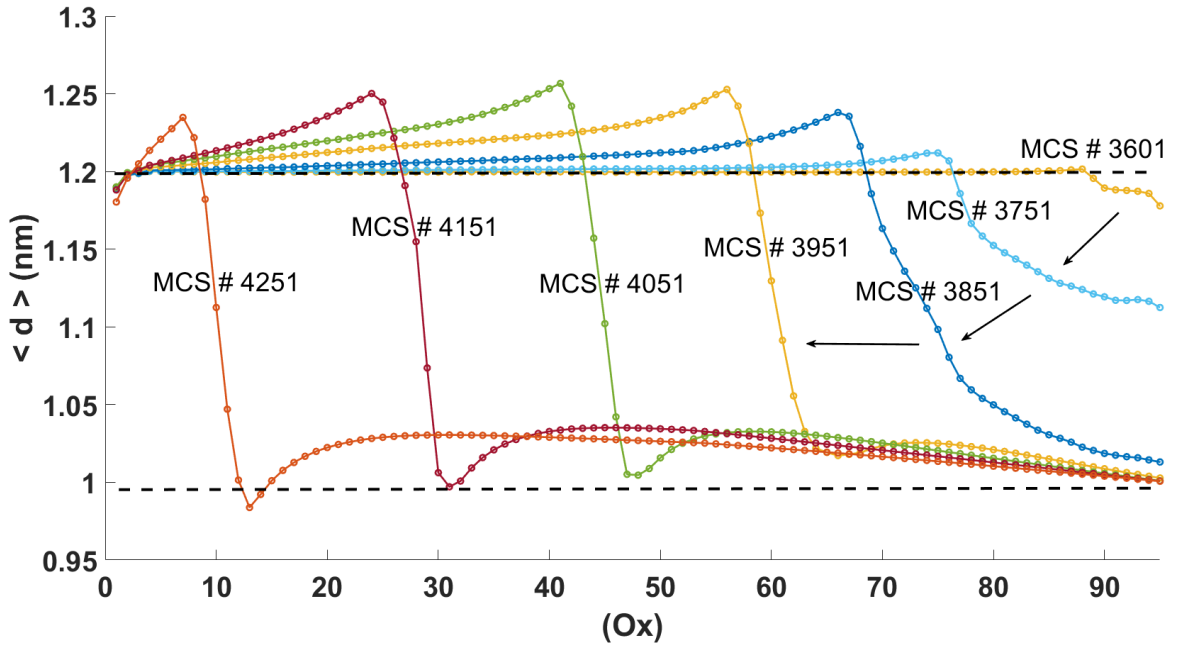
(a) Elastic interface profiles corresponding to the Euclidean distance between two successive spins. The dashed lines represent the equilibrium 1n distances R_0^{HH} = 1.20 nm and R_0^{LL} = 1.00 nm.
