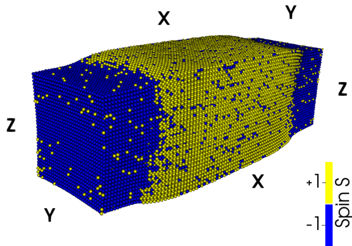
(b) n_{HS} = 0.57 at T = 78K
