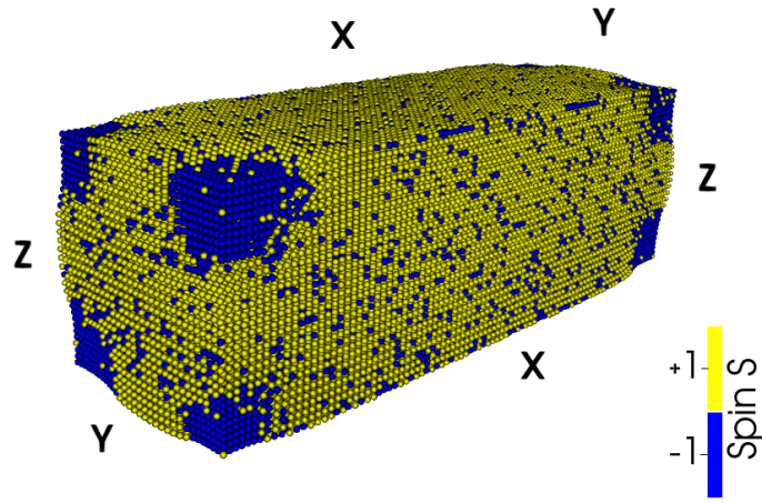
(a) n_{HS} = 0.87 at T = 79K
