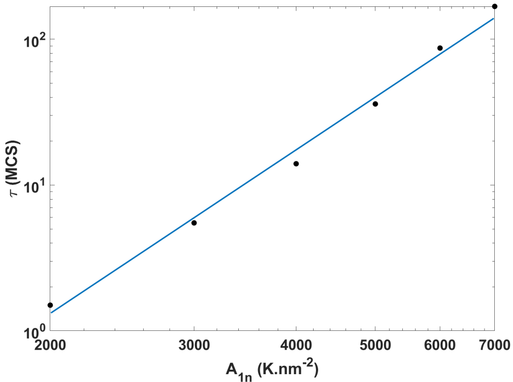
Figure 12 – Variation, in log-log scale, of the lifetime of the metastable state \tau , evaluated at n_{HS} = \frac{1}{2} in Figure 11)a as a function of A_{1n} , which fits with the linear regression (blue curve) with a slope \alpha \simeq 4.4 , suggesting the power law \tau \sim (A_{1n})^{4.4} .
