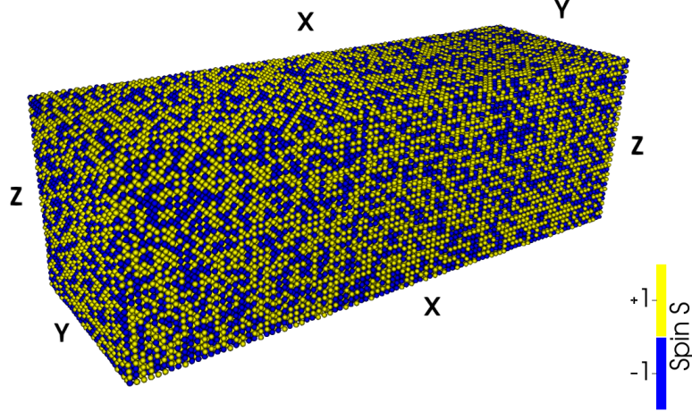
Figure 6 – Snapshot showing the spatiotemporal configurations of the lattice during the cooling branch at n_{HS} = 0.55 and T = 92K for A_{1n} = 50 . Yellow (blue) spheres represent HS (LS) sites.
