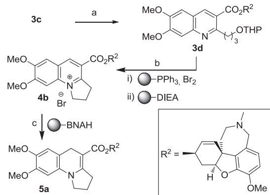
Scheme 3. Reagents and conditions: a) Galantamine, HATU, DIEA, DMAP, \text{CH}_2\text{Cl}_2 , 25^\circ\text{C} , 16 h (85%); b) (i) PS- \text{PPh}_3 , \text{Br}_2 , \text{CH}_2\text{Cl}_2 , 36 h, (ii) PS-DIEA, 48 h (70%); c) PS-BNAH, \text{CH}_2\text{Cl}_2 , 25^\circ\text{C} , 6 h, (100%).
