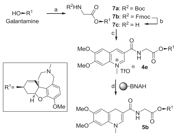
Scheme 7. Reagents and conditions: a) N -Boc-Gly, HATU, DIEA, CH 2 Cl 2 , 25 °C (76%) for 7a or N -Fmoc-Gly, HBTU, DMAP, CH 2 Cl 2 , 25 °C, 16 h (74%) for 7b ; b) piperidine, CH 2 Cl 2 , 25 °C, 2 h (88%); c) (i) 4d , CH 2 Cl 2 , 25 °C, 30 min, (ii) Si-carbonate, 1 h (89%); d) PS-BNAH, CH 2 Cl 2 , 25 °C, 3 h, 95%.
