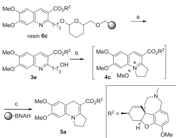
Scheme 5. Reagents and conditions: a) PPTS, 1,2-dichloroethane/ n -butanol, 60 °C, 16 h; b) MsCl, acetone, K 2 CO 3 , -30 °C → 20 °C, 1h30; c) PS-BNAH, CH 2 Cl 2 , 25 °C, 6 h.
