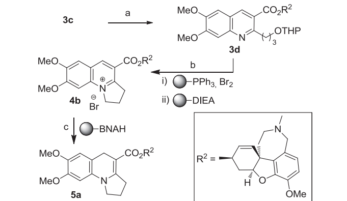
Scheme 3. Reagents and conditions: a) Galantamine, HATU, DIEA, DMAP, \text{CH}_2\text{Cl}_2 , 25^\circ\text{C} , 16 h (85%); b) (i) PS- \text{PPh}_3 , \text{Br}_2 , \text{CH}_2\text{Cl}_2 , 36 h, (ii) PS-DIEA, 48 h (70%); c) PS-BNAH, \text{CH}_2\text{Cl}_2 , 25^\circ\text{C} , 6 h, (100%).
