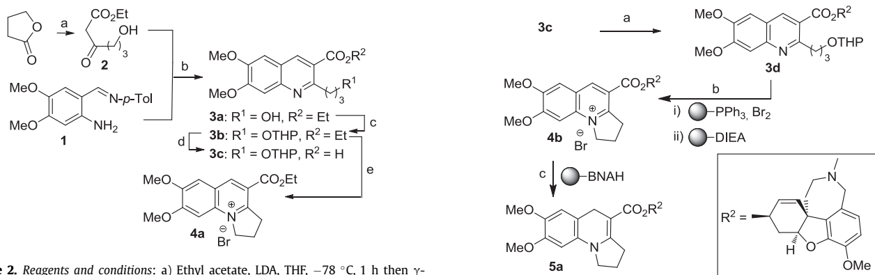
Scheme 3. Reagents and conditions: a) Galantamine, HATU, DIEA, DMAP, \text{CH}_2\text{Cl}_2 , 25^\circ\text{C} , 16 h (85%); b) (i) PS- \text{PPh}_3 , \text{Br}_2 , \text{CH}_2\text{Cl}_2 , 36 h, (ii) PS-DIEA, 48 h (70%); c) PS-BNAH, \text{CH}_2\text{Cl}_2 , 25^\circ\text{C} , 6 h, (100%).
