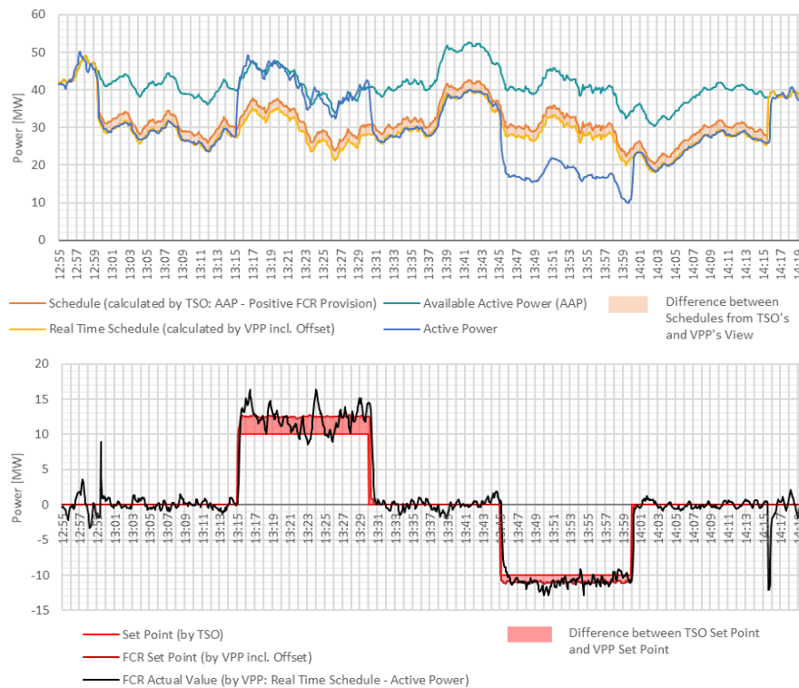
Fig. 4: Flexibility dispatch, absolute (above) and relative (below).
