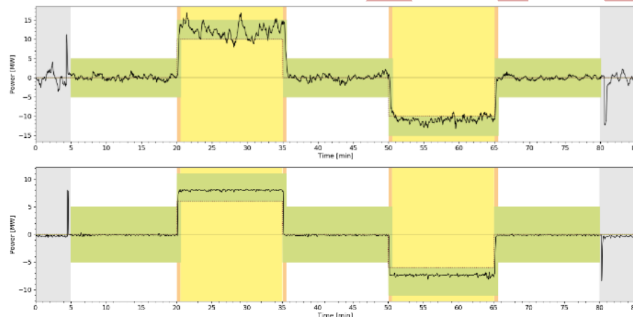
Fig. 6 : Comparison of two tests: #2 (above) and #1 (below) according to the tolerance corridors for FCR.
