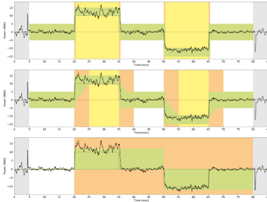
Fig. 7 : Fulfilment corridor for FCR (above), aFRR (middle) and mFRR (below) during the 3rd full-test of the VPP
