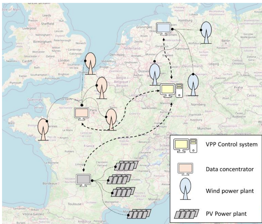
Fig. 1: Physical architecture of the VPP
