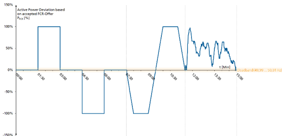
Fig. 5: General test schedule characterised by series of positive and negative symmetrical reserve activations
