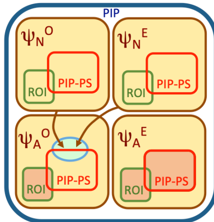
Figure 1. Classification of the different ontological models assuming the PIP (see text). \psi_N^O and \Psi_N^E models can be transformed (see arrows) into models of the \psi_A^O class (blue ellipse domain). Models satisfying PIP-PS (red boxes) and ROI (green boxes) are also represented. Dark orange regions are prohibited by no-go theorems: \psi_A^E models assuming PIP-PS are excluded by the PBR theorem [4], whereas the ROI domain in the \Psi_A regions are excluded by the H-ROI (II) theorem derived in this work. Note, that the models prohibited by the original H-ROI theorem [6] are inside the ROI subdomain of the \psi_A^E class.
