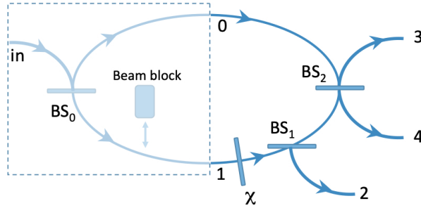
Figure 2. Principle of the interferometric proof for the H-ROI theorem [6]. BS_i ( i = 0, 1, 2 ) denote beam-splitters, and paths/gates are labeled as indicated in the figure (see main text). A phase-shifter ( \chi ) is introduced in path 1. The sketch also includes (light blue color region in the dashed box) the preparation stage (with a movable beam-blocker) which is used to modify the original proof given in [6].
