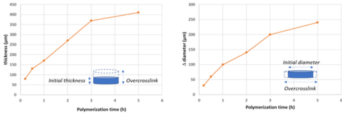
Fig. 4. Evolution with polymerization time of a) thickness and b) \Delta diameter (diameter at time t – original diameter) of a photo-cured cylinder obtained after 60 s irradiation of the formulation PCL-300/DOD-BisTMC/TX-TBD = 10/100/5 using a Max X43 DLP apparatus from ASIGA.
