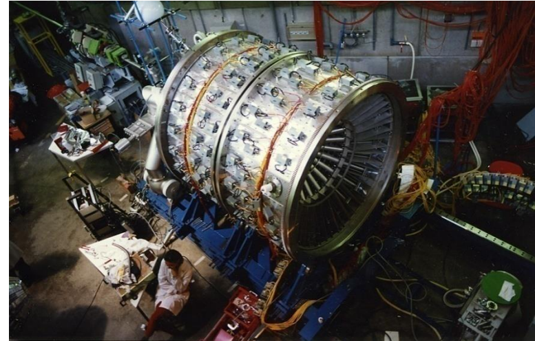
CATANE DETECTOR
