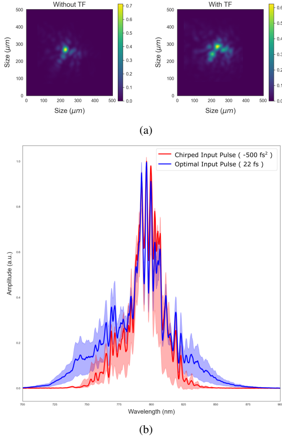
Figure 3: Measured focus images (a) and pulse spectra (b). In (a), the left image shows the reference focus with no glass films in the beam path and the right image shows the focus after the thin films have been installed. For (b), the red spectrum is the average of 2 initial shots that result when the input pulse is chirped before entering the glass films and leads to no broadening due to the decrease in the pulse intensity. The blue spectrum shows the average value of 36 shots when the input pulse duration is optimized to 22 fs duration with maximum pulse intensity so that nonlinear spectral broadening occurs in the plate. The red and blue shaded regions represent their respective standard deviations.
