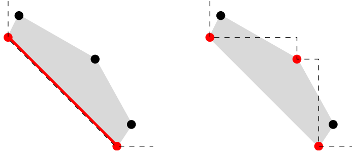
Figure 2: Multi-objective optimization over a polygon K \subset \mathbb{R}^2 , and over its vertices. Left: Pareto front of the problem \min_{x \in K}(x_1, x_2) . Right: Pareto front of the problem \min_{x \text{ vertex of } K}(x_1, x_2) . Note that the second Pareto front is not included in the first one.
