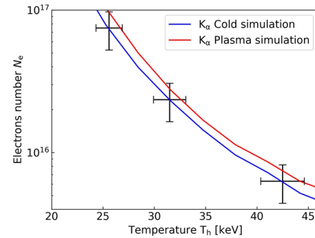
FIG. 8. Parameters T_h and N_e that reproduce the K_{\alpha} signal on the ZnVH spectrometer in the experiment from Ref. 16 according to Geant4 simulations. The blue curve is from the nominal Geant4 simulation (i.e., a cold target composed of 175 \mu\text{m} CH and 20 \mu\text{m} Cu), and the red curve is for the plasma case. The Geant4 library used to compute the K_{\alpha} was Livermore. The predicted hot-electron temperatures are \sim 5\% greater for the plasma case than for the cold case, while the difference in the parameter N_e does not exceed 30%. These percentages are indicated by the error bars.
