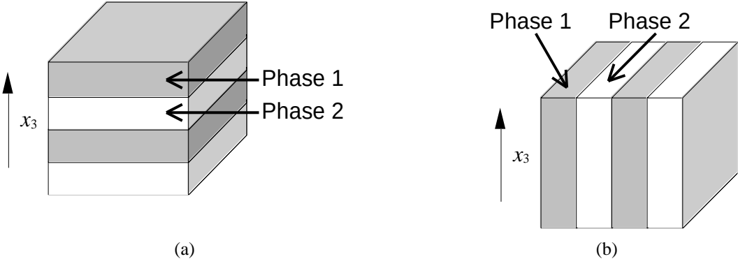
Figure 1 – Basic piezocomposite cell for the 2-2 (a) series and (b) parallel connectivities.
