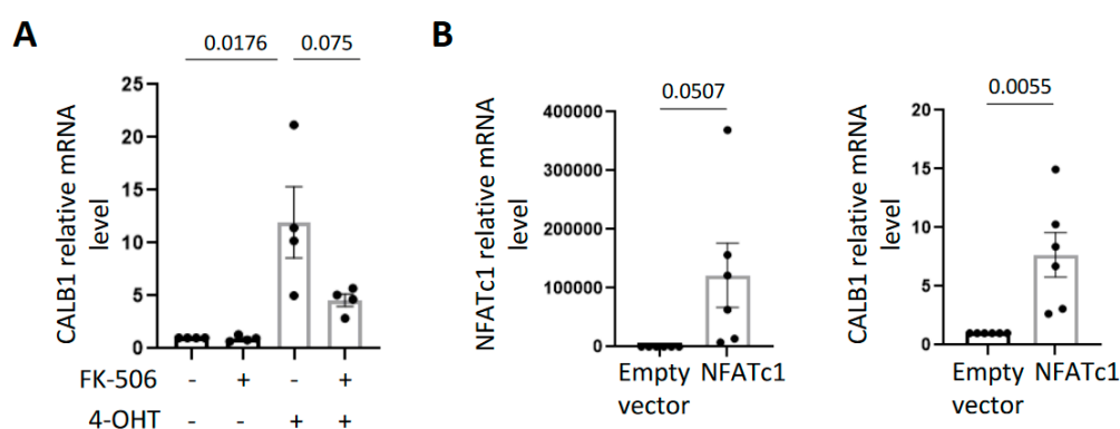
Figure 3. The calcium-dependent calcineurin/NFAT pathway induces CALB1 expression upon oncogene activation in HMECT. (A) CALB1 mRNA level was measured by RT-qPCR in HMECT overexpressing 4-OHT-inducible Mek:ER and treated (+) or not (−) with FK-506, a calcineurin inhibitor (treated every day with 2 \mu\text{M} during six days), or/and with 4-OHT (100 nM). The first three days, cells were co-treated with 4-OHT and FK-506 (first treatment 4 h prior 4-OHT), and the three last days only with FK-506. Mean \pm SEM of four independent experiments are shown. An unpaired t -test was performed and p -value is indicated. (B) NFATc1 ( left panel) and CALB1 ( right panel) mRNA levels were measured by RT-qPCR in HMECT 24 h after infection with a vector encoding NFATc1 or control empty vector. Mean \pm SEM of six independent experiments are shown. Unpaired t -tests were performed, and p -values are indicated.
