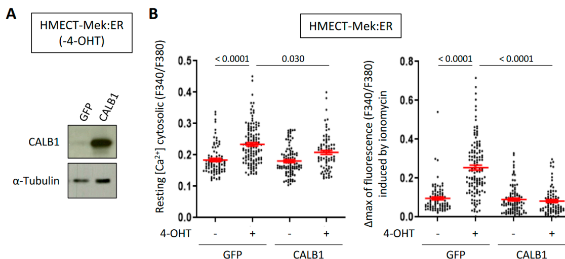
Figure 4. CALB1 overexpression buffers increased \text{Ca}^{2+} levels induced by oncogene activation in HMECT. (A) CALB1 protein level was assessed by Western Blot in HMECT-Mek:ER (without 4-OHT) infected with a vector encoding CALB1 or the corresponding GFP control vector. \alpha -Tubulin protein level was assessed as a loading control. (B) \text{Ca}^{2+} levels were measured with the ratiometric probe Fura2 in HMECT-Mek:ER inducible oncogene and CALB1 or the corresponding GFP control vector, with or without 4-OHT treatment. Resting cytosolic \text{Ca}^{2+} concentration was evaluated as a stable fluorescent ratio before stimulation ( left panel), and the size of \text{Ca}^{2+} intracellular stocks was estimated as the \text{Ca}^{2+} peak amplitude obtained after ionomycin stimulation ( right panel). Means \pm SEM of 3 independent experiments are presented. Kruskal–Wallis test was performed, and p -values are indicated. Three days after 4-OHT treatment, GFP- 4-OHT n = 85 or + 4-OHT n = 126 , CALB1- 4-OHT n = 99 or + 4-OHT n = 77 .
