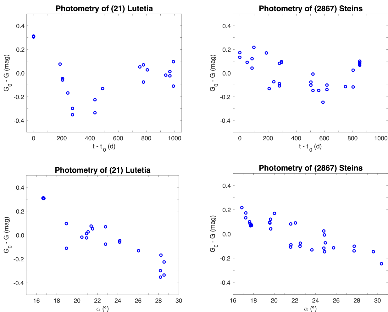
Fig. 27: Observed G magnitudes of asteroid (21) Lutetia included in Gaia DR3, relative to the mean of the magnitudes ( G_0 ), as a function of days after the first observation ( t_0 ) (top left). The top right panel shows the same as the left panel for (2867) Šteins. The bottom panel shows the same as the top panel, but the magnitudes are depicted against the phase angle.
