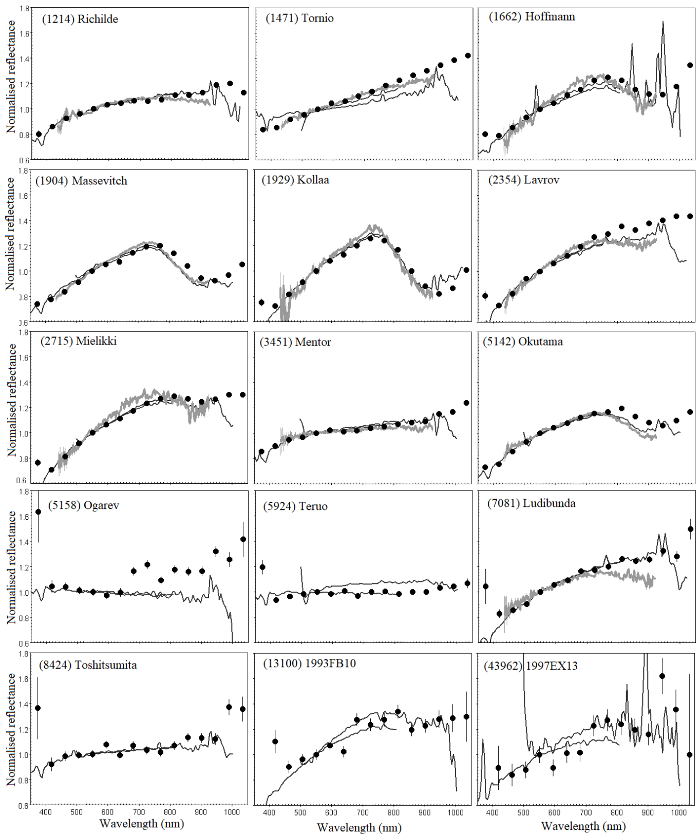
Fig. G.2. Gaia 's mean reflectance spectra (black circles) against ground-based observations; Cellino et al. (2020) spectra in dark grey lines and those of (Bus & Binzel 2002b) in light grey lines for asteroids (1214), (1471), (1662), (1904), (2354), (2715), (3451), (5142), (7081).
