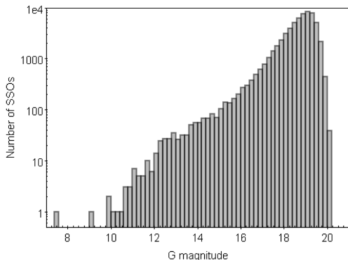
Fig. 2. G-magnitude distribution of SSOs with reflectance spectra.
