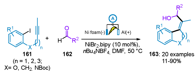
Scheme 30. Intramolecular Carbonickelation of Alkynes and Subsequent Reaction with Aldehydes
