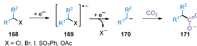
Scheme 31. Two Consecutive SET Electroreductions and Subsequent Carboxylations
