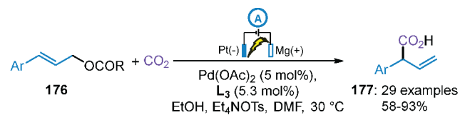
Scheme 32. Pd-Catalyzed Electroreductive Carboxylation of Allylic Esters
