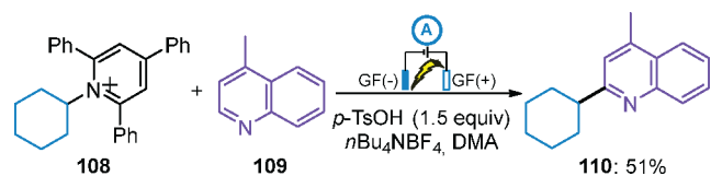
Scheme 19. Electrochemical Deaminative Minisci-Type Alkylation of Quinoline 109 with Kratritzky Salt 108
