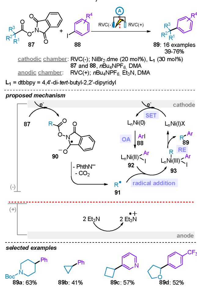
Scheme 16. Ni-Catalyzed Electroreductive Cross-Coupling between NHP Esters and Aryl Iodides
