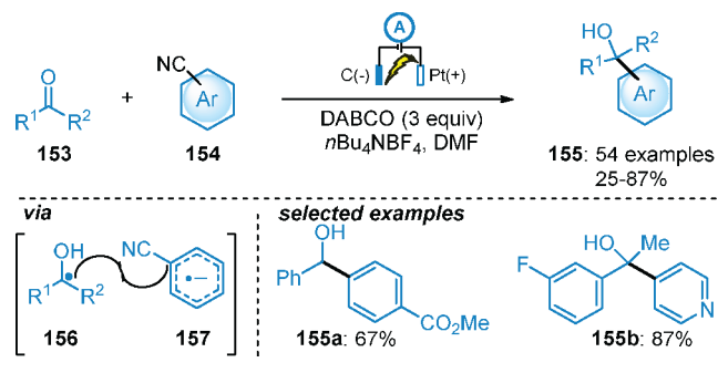
Scheme 28. Electroreductive Coupling between Carbonyl Compounds and Cyano(aza)arenes
