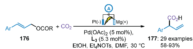
Scheme 32. Pd-Catalyzed Electroreductive Carboxylation of Allylic Esters
