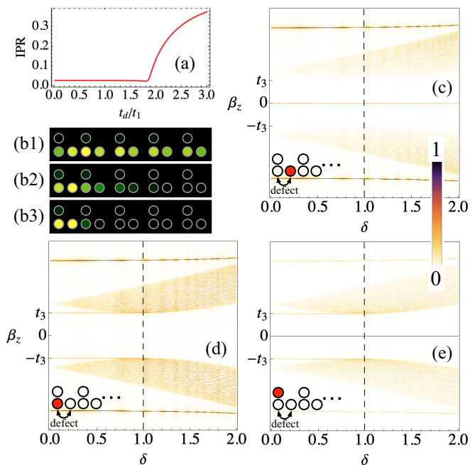
FIG. 6. (a) Inverse participation ratio (IPR) vs t_d/t_1 for both Tamm states, for \delta = 1.4 and t_3 = 1 . (b1)–(b3) Intensity profiles for Tamm states for t_d/t_1 = 1.85, 2.1, and 3.0 , for the same parameters used in (a) and using an avocado color scale. (c)–(e) Frequencies excited vs \delta , for A-, B-, or C-edge input conditions, as sketched in the insets. Simulations were performed considering 31 unit cells and a propagation length of z_{\max} = 1000 .
