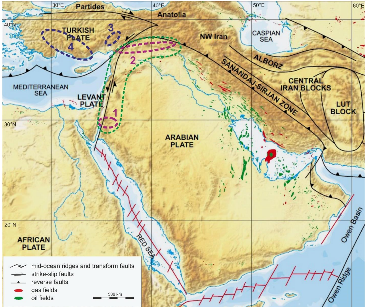
Fig. 1. Regional Map and tectonic setting in the Middle East. Levant region is framed by green broken line. The discussed areas in the southern and in the northern Levant are indicated by purplecoloured ellipses (1 – southern Levant / southern Jordan, 2 – northern Levant and South Anatolian Autochthon Belt / Border Folds); Taurid regions are indicated by blue-coloured ellipses (3 – eastern Taurides, 4 – western Taurides). Reproduced from Sharland et al. (2001) with permission of Gulf Petrolink.
