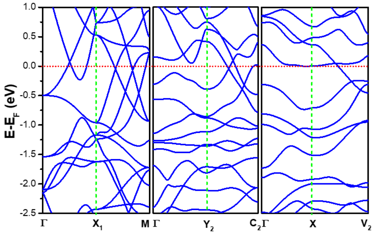
Figure 6. Effects of oxygen doping on energy bands of \beta -W. (a) – (c) show the energy bands for the unit cells of undoped, one O doped, and two O doped \beta -W, respectively, considering nearly equivalent directions in the respective Brillouin zones.
