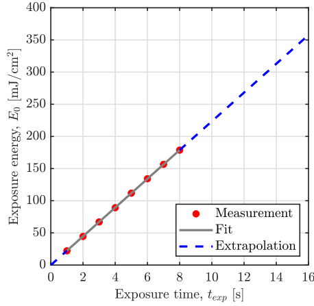
Fig. 11 Relation between the exposure time and UV light energy on the PDMS window of the EMBER 3D DLP printer measured by G&R Labs Model 222 light meter.
